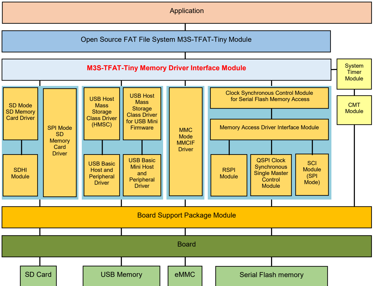
Fig.1-1 Structure of software
