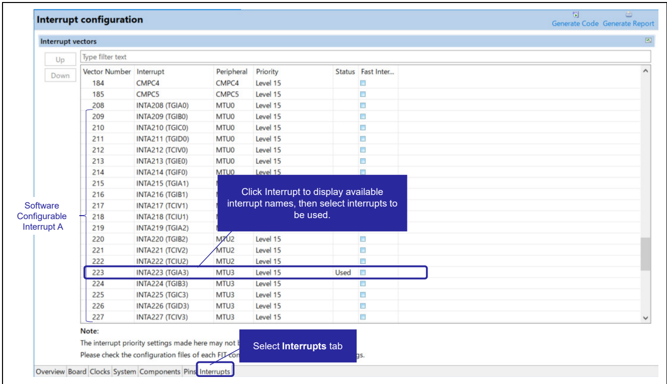
Figure 3.5 Interrupt Settings
