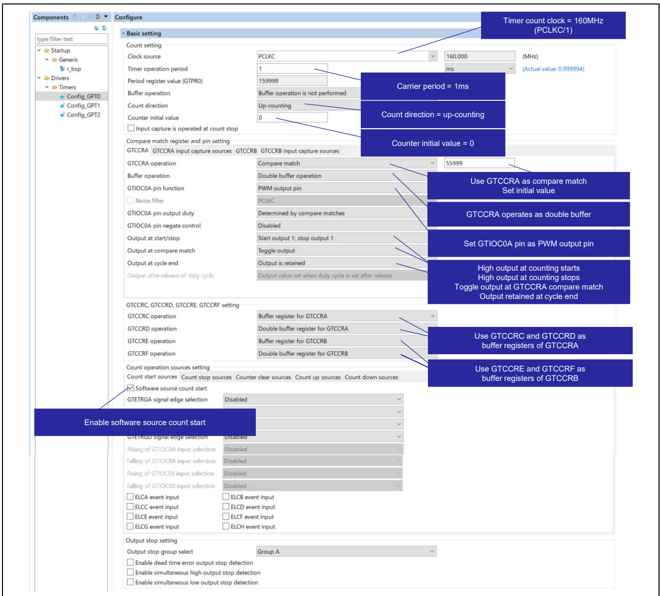
Figure 4.33 GPT0 Settings (1/2)
