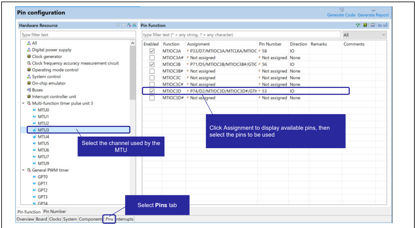
Figure 3.4 Pin Settings
