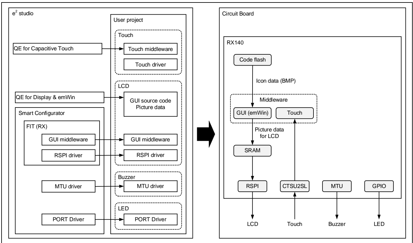
Figure 1-3 Software configuration
