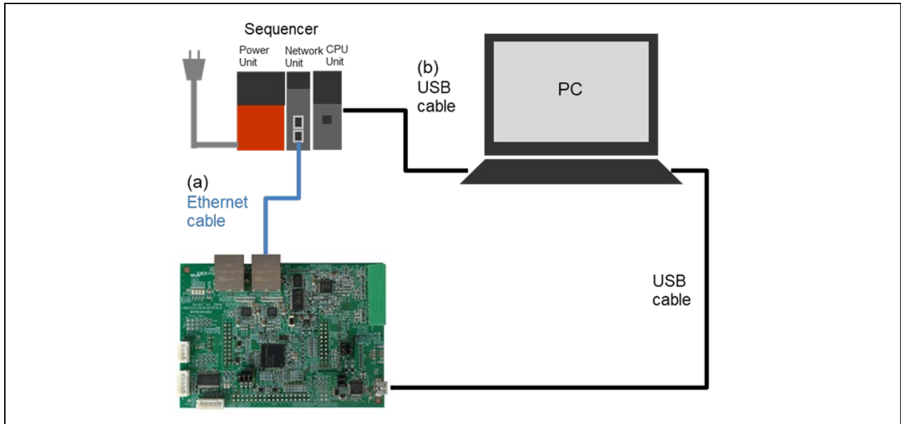
Figure 6.1 Connection configuration
