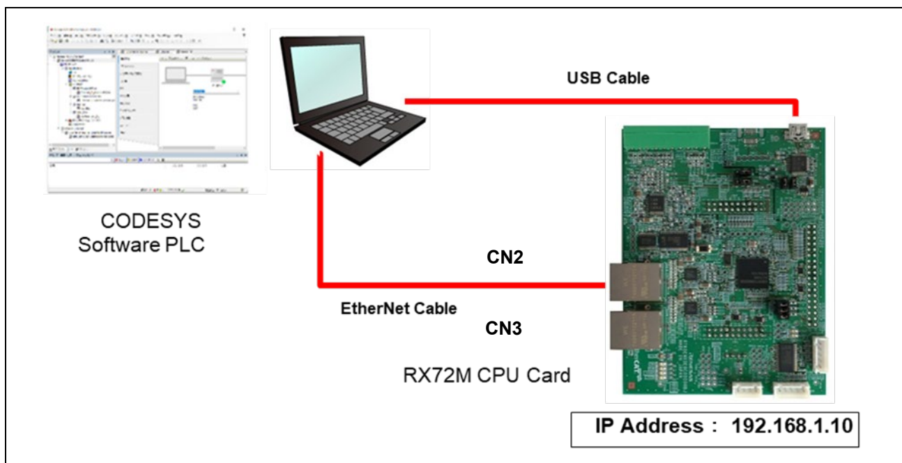
Figure 5.1 Connection configuration
