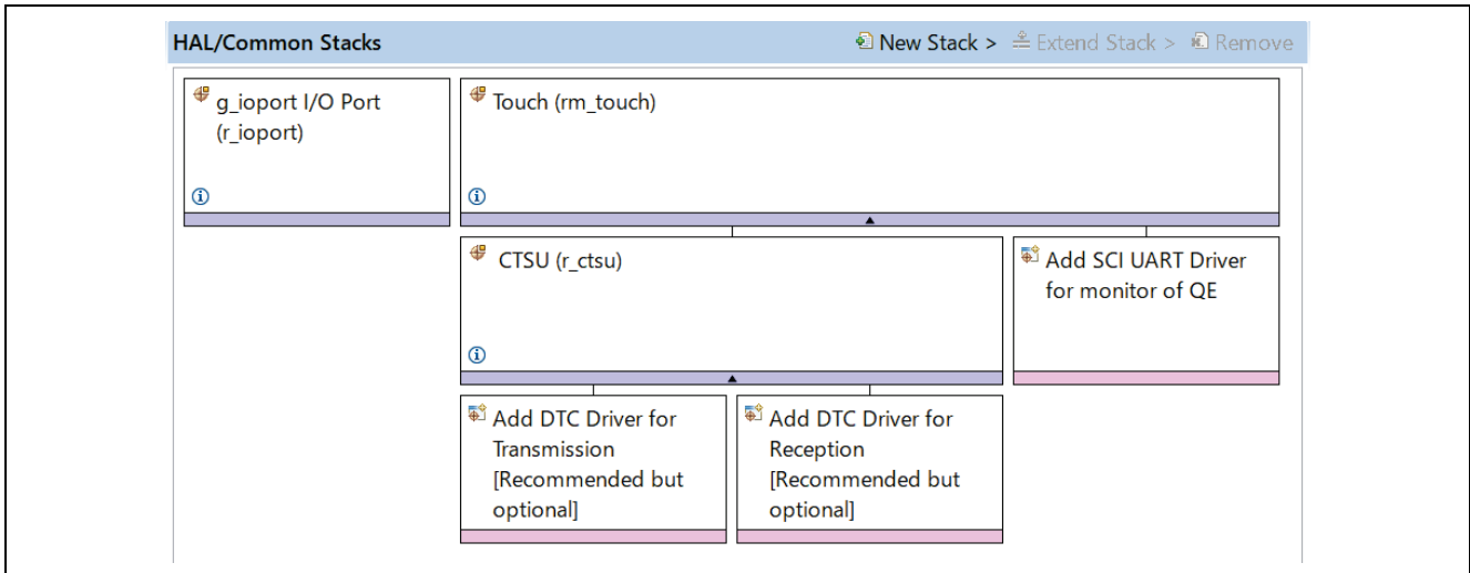
Figure 21. HAL/Common Stacks (after CTSU is added)
