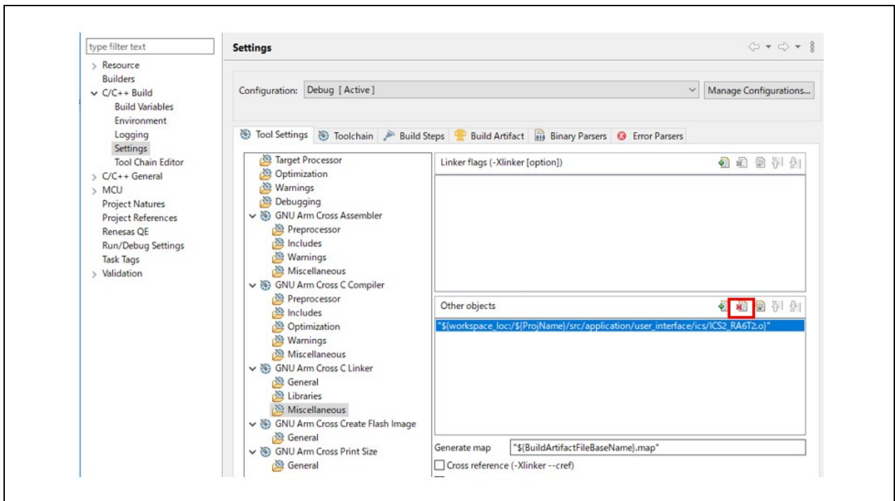
Figure 4-20 Unregister ICS2_RA6T2.o
