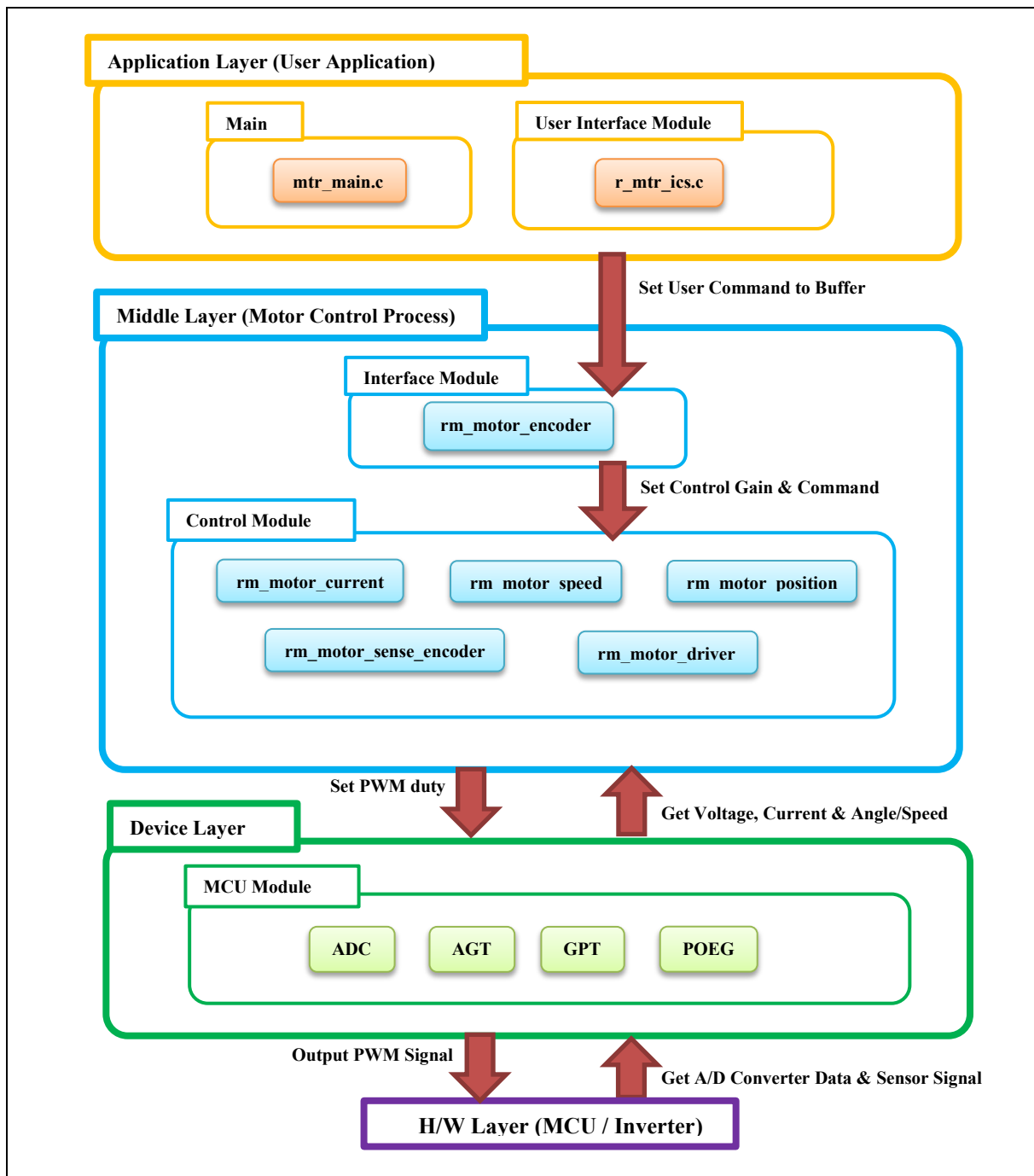
Figure 2-50 Module Configuration
