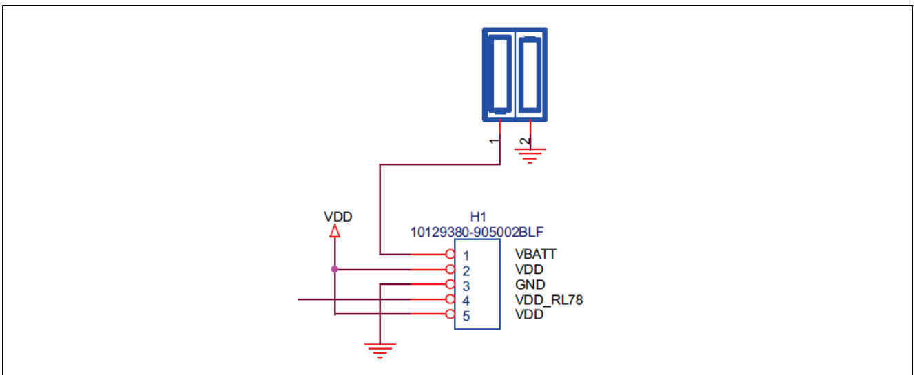
Figure 32. H1 Schematic
