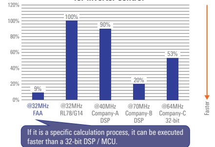
Comparison of processing time of PI calculations for inverter control
