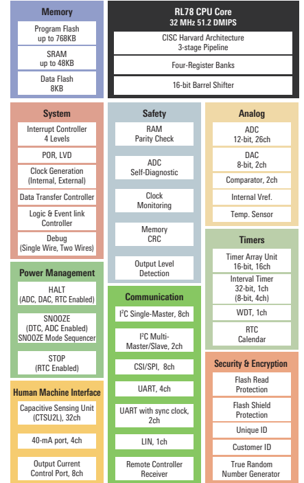
Note: The block diagram of G23
