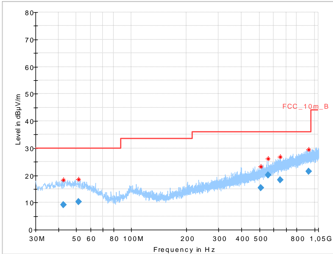
Plot 3: 30 MHz to 1 GHz, TX mode, 2480 MHz, vertical & horizontal polarization, 1 Mps
