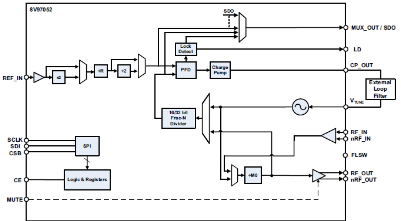
Figure 1. Block Diagram
