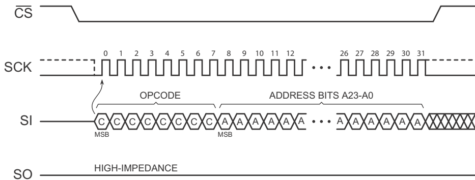
Figure 34. Sector Erase Sequence Diagram
