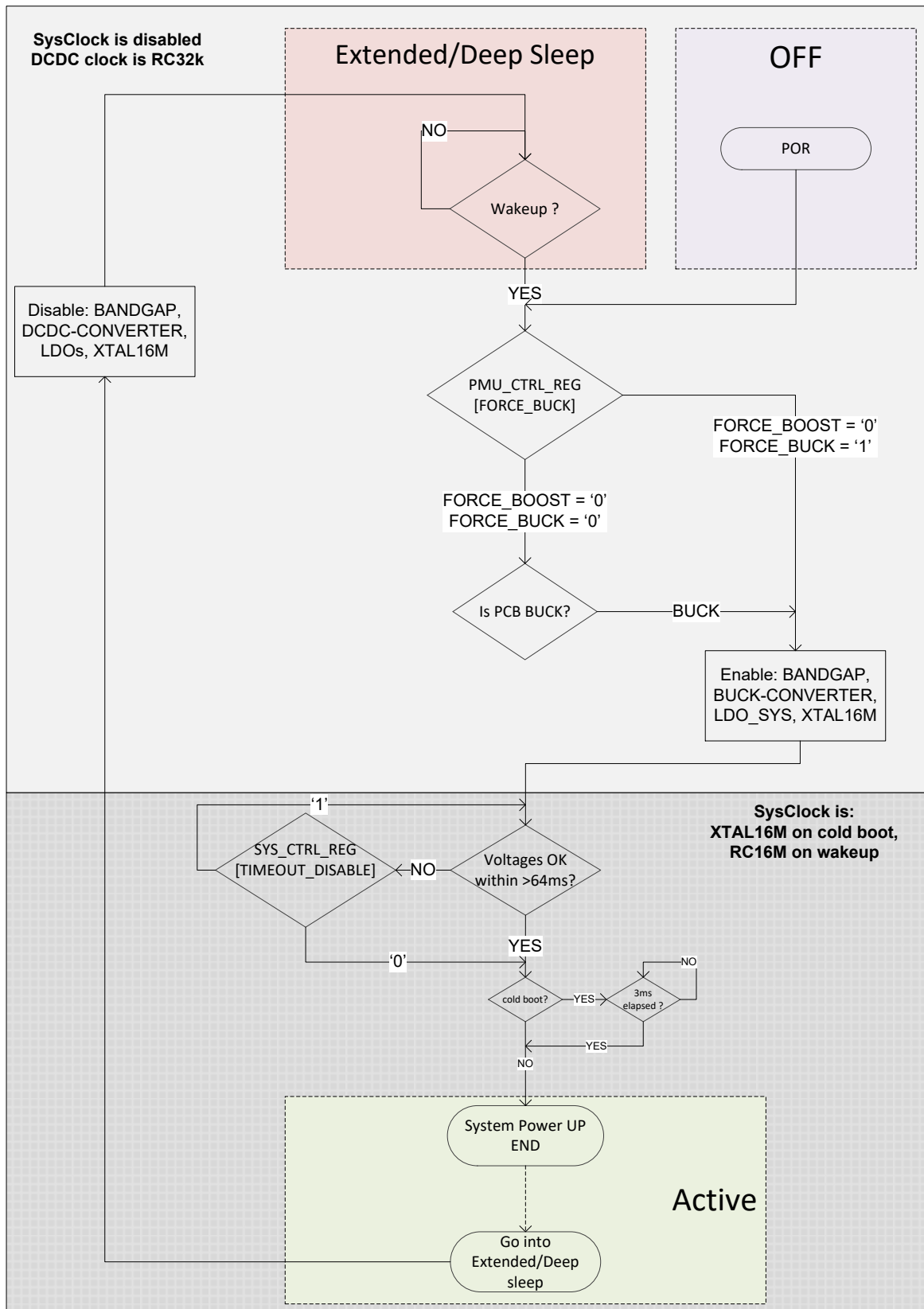
Figure 7: Power/Wake-Up Sequence
