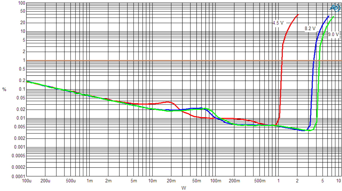
Figure 3. THD versus continuous output power (8 Ω + 33 μH)
