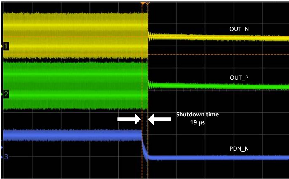
Figure 10. Shutdown timing (19 \mu s from de-asserting PDN_N to zero output)
