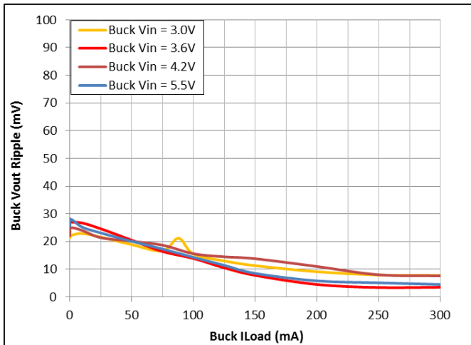
Figure 19: Buck V_{OUT} = 0.9\text{ V}
