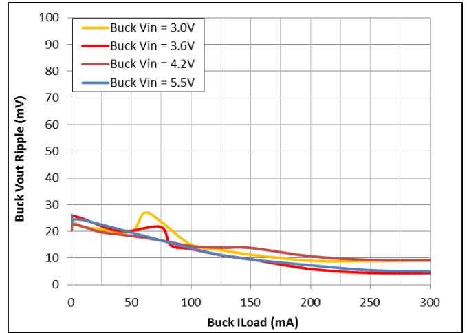
Figure 18: Buck V_{OUT} = 1.3\text{ V}
