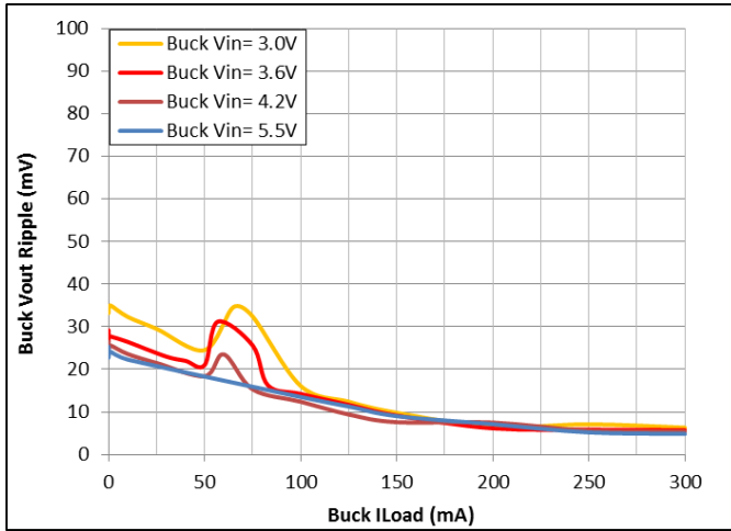
Figure 17: Buck V_{OUT} = 1.9\text{ V}
