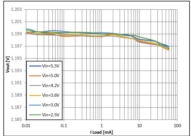
Figure 21: Buck V_{OUT} = 1.2\text{ V}
