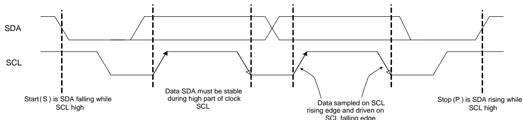
Figure 37: I 2 C Start and Stop Conditions
