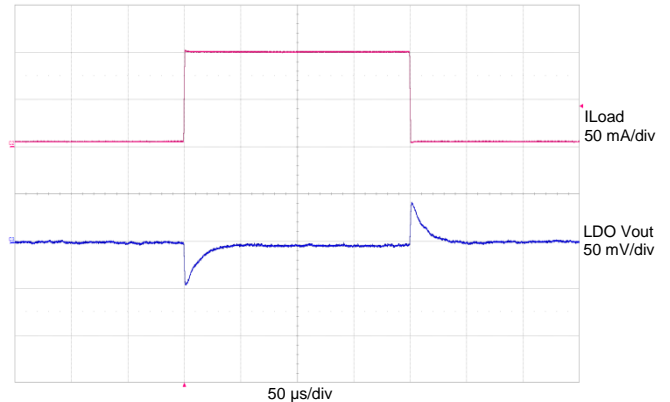
Figure 145: LDO I_{LOAD} = 5 \text{ mA} to 100 \text{ mA} to 5 \text{ mA} ( 0.1 \text{ A} / 1 \mu\text{s} ); LDO V_{IN} = 3.6 \text{ V} , LDO V_{OUT} = 2 \text{ V}
