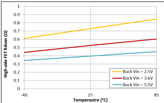
Figure 6: High-Side FET
