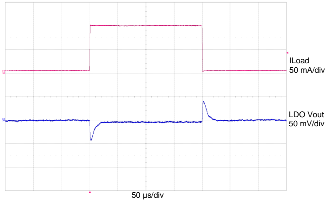
Figure 134: LDO I_{LOAD} = 5 \text{ mA} to 100 \text{ mA} to 5 \text{ mA} ( 0.1 \text{ A} / 1 \mu\text{s} ); LDO V_{IN} = 3.6 \text{ V} , LDO V_{OUT} = 0.8 \text{ V}
