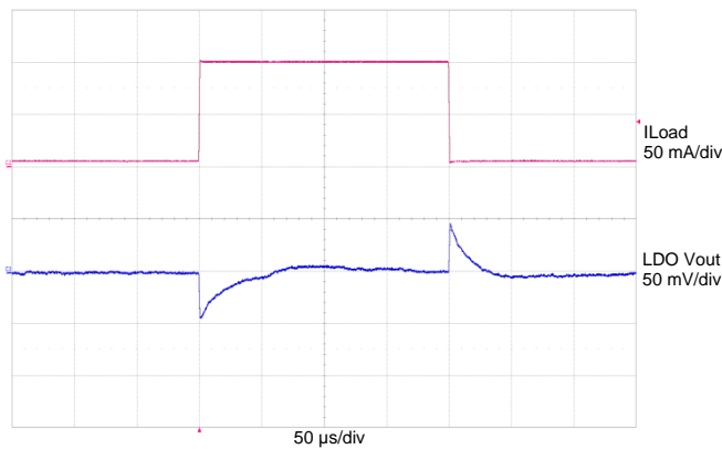
Figure 156: LDO I_{LOAD} = 5 \text{ mA} to 100 \text{ mA} to 5 \text{ mA} ( 0.1 \text{ A} / 1 \mu\text{s} ); LDO V_{IN} = 3.6 \text{ V} , LDO V_{OUT} = 3.3 \text{ V}
