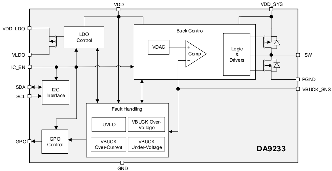
Figure 1: Block Diagram
