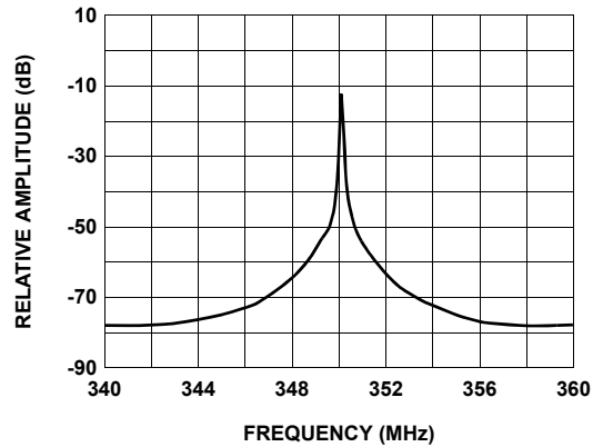
FIGURE 18. OUTPUT SPECTRUM - WIDEBAND
