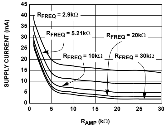
FIGURE 8. SUPPLY CURRENT vs R_{RAMP}
