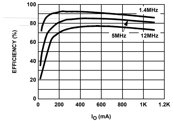
FIGURE 10. EFFICIENCY vs I_O (PWM MODE)
