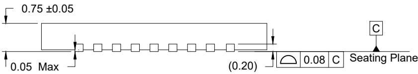
SIDE VIEW
