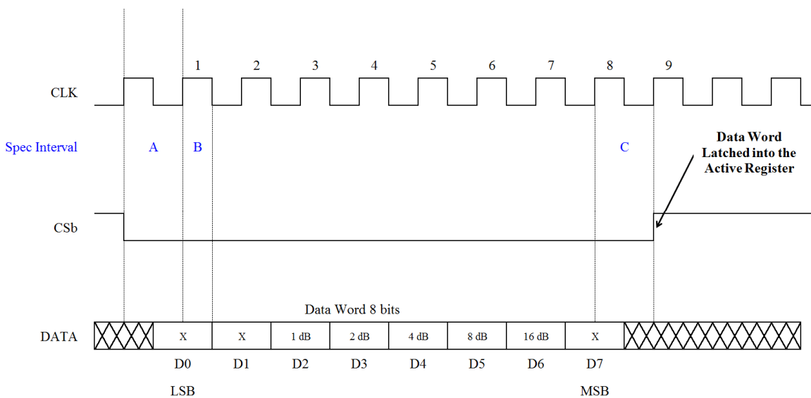
SERIAL REGISTER TIMING DIAGRAM: (Note the Timing Spec Intervals in Blue )
