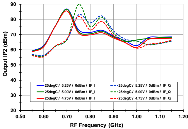
IP 2O vs. V CC [Low Side Injection]
