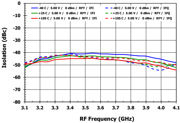
RF Switch Isolation
