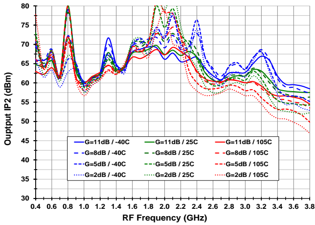
Figure 16. Output IP2 vs. Temperature and Gain Setting
