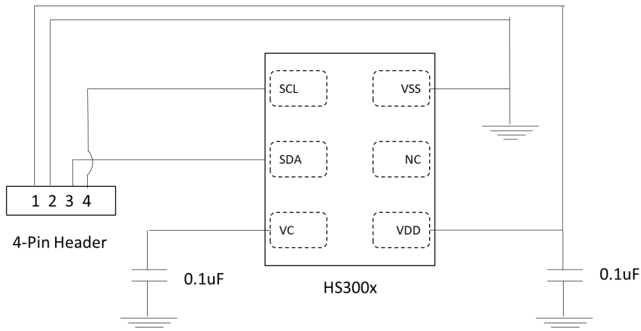
Figure 2. HS3xxx-ML1 PCB Schematic
