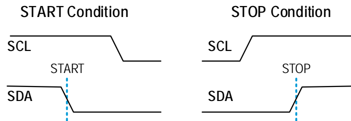
Figure 12. START and STOP Condition Waveform
