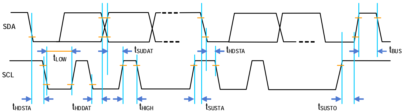
Figure 11. Timing Diagram
