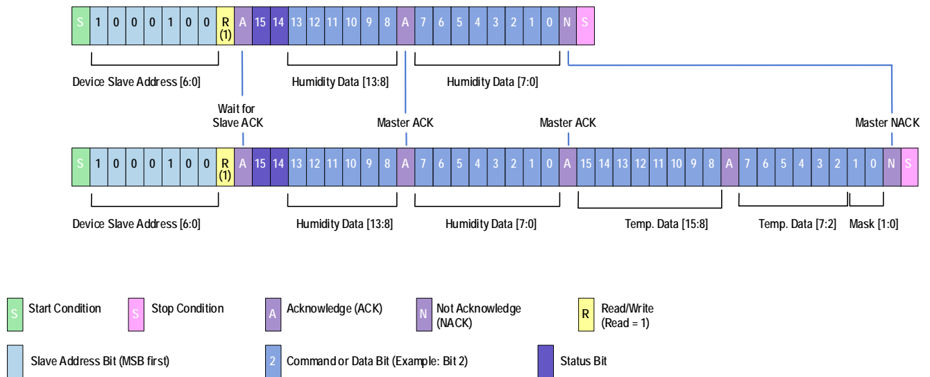
Figure 14. Data Fetch
