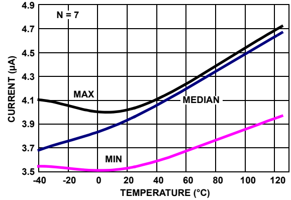
FIGURE 26. ISL28276 SUPPLY CURRENT vs TEMPERATURE, V_+, V_- = \pm 2.5V DISABLED, R_L = INF
