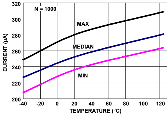
FIGURE 25. ISL28476 SUPPLY CURRENT vs TEMPERATURE, V_+, V_- = \pm 2.5V ENABLED, R_L = INF
