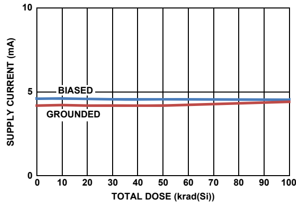
FIGURE 7. TOTAL SUPPLY CURRENT vs RADIATION
