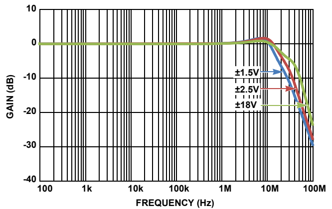
FIGURE 42. SUPPLY VOLTAGE vs FREQUENCY RESPONSE
