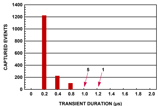
FIGURE 2. TYPICAL SINGLE EVENT TRANSIENT DURATION AT +25 ^\circ\text{C} LET = 60MeV \cdot cm 2 / mg IN UNITY GAIN ( V_S = \pm 18\text{V} )
