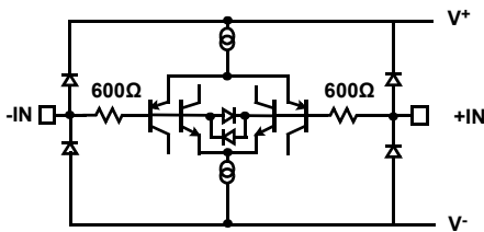
CIRCUIT 1
