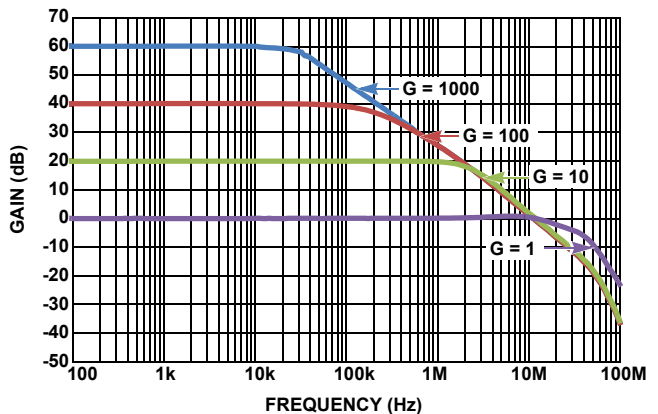
FIGURE 38. CLOSED LOOP GAIN vs FREQUENCY RESPONSE
