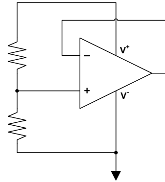
FIGURE 66. PREVENTING OSCILLATIONS IN UNUSED CHANNELS, SINGLE SUPPLY
