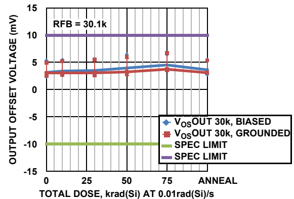
FIGURE 14. V_{0sOUT} (GAIN = 1) vs TOTAL DOSE
