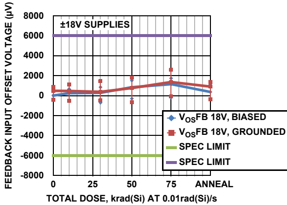
FIGURE 9. V_{0sFB} vs TOTAL DOSE
