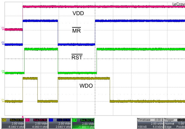
Figure 14. ISL7x6xEH Start-Up to RESET, Manual RESET, and \overline{\text{WDO}} Function
