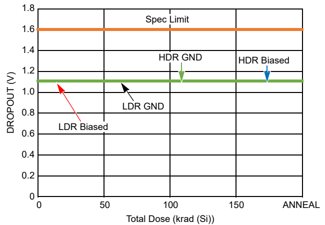
Figure 11. Dropout Shift
