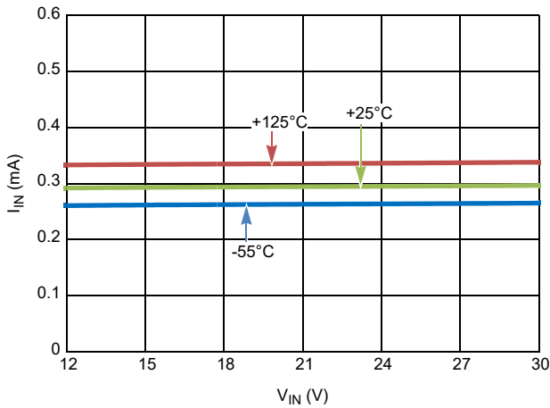
Figure 18. I_{IN} vs V_{IN} Over Temperature
