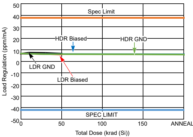
Figure 10. Load Regulation (Sinking) Shift
