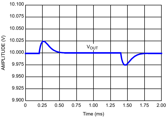
Figure 29. Simulated Load Transient ( \Delta I_L = 1\text{mA} )
