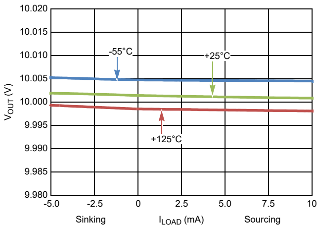
Figure 14. Load Regulation vs V_{OUT} (V) Over Temperature
