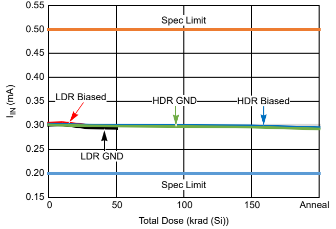
Figure 7. Supply Current Shift
