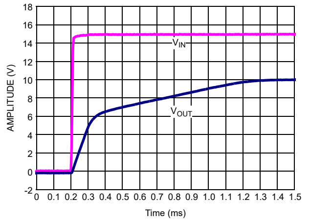
Figure 21. Turn-On Time
