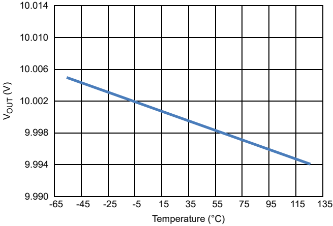
Figure 25. Simulated (Worse Case) V_{OUT} vs Temperature
