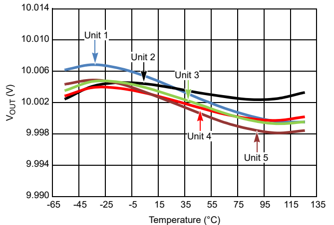
Figure 17. V_{OUT} vs Temperature
