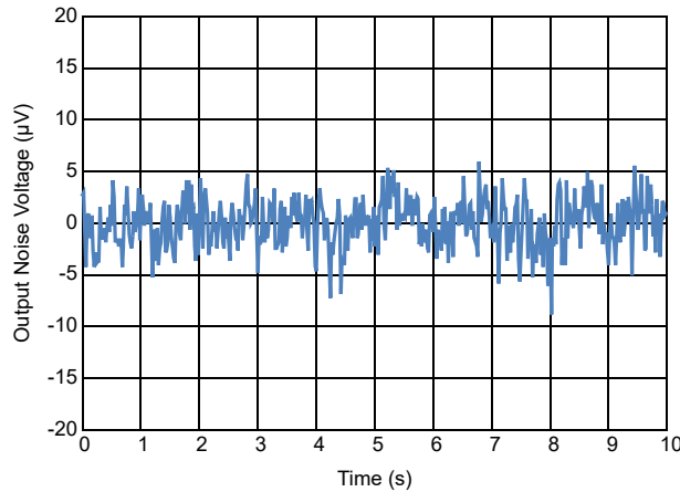
Figure 24. V_{OUT} vs Noise, 0.1Hz to 10Hz
