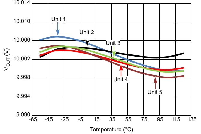
Figure 26. Characterized V_{OUT} vs Temperature
