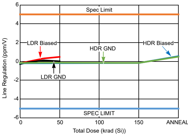
Figure 8. Line Regulation Shift
