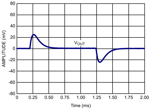
Figure 20. Load Transient ( \Delta I_L = 1mA )
