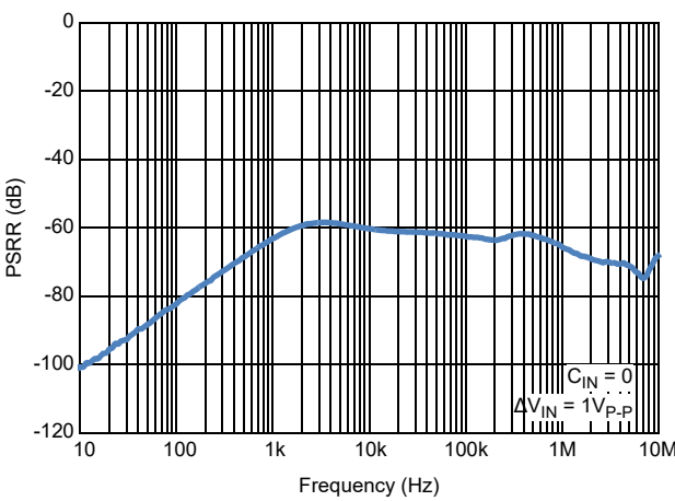
Figure 22. Ripple Rejection vs Frequency
