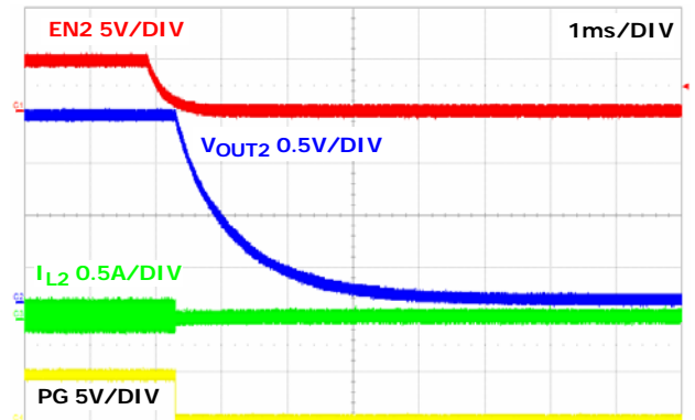
FIGURE 31. SOFT-DISCHARGE SHUTDOWN CHANNEL 2
