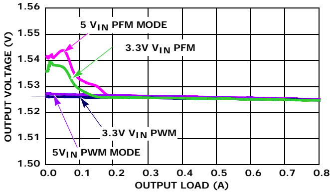
FIGURE 8. V_{OUT} REGULATION vs LOAD 2.25MHz 1.5V OUT
