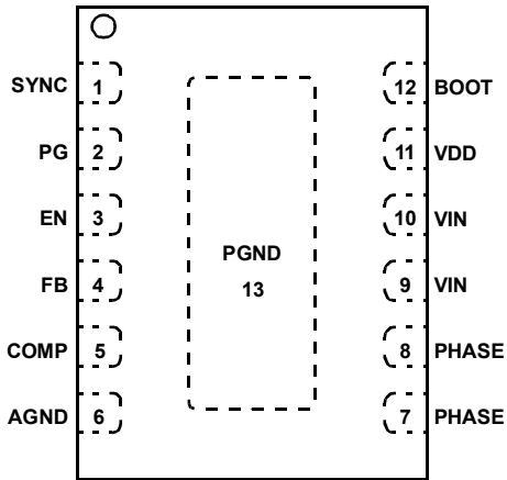
ISL85003 (12 LD 3X4 DFN) TOP VIEW
