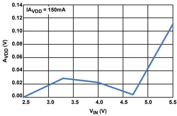
FIGURE 3. A_{VDD} LINE REGULATION vs V_{IN}
