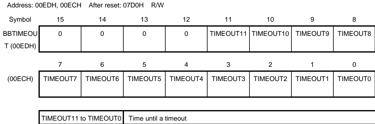
Figure 4-75 Format of Reception Timeout Register (BBTIMEOUT)
