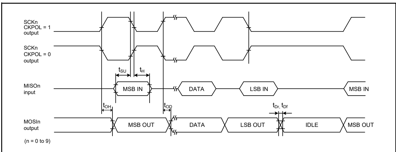
Figure 2.44 SCKn simple SPI mode timing for master when CKPH = 0
