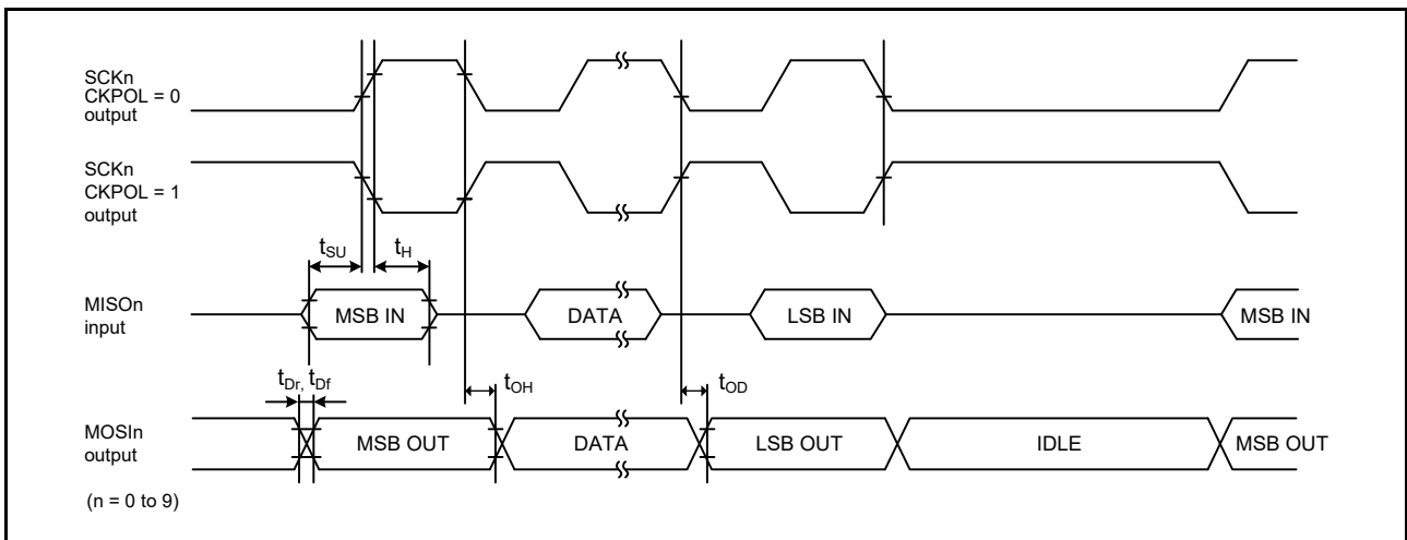
Figure 2.43 SCKn simple SPI mode timing for master when CKPH = 1
