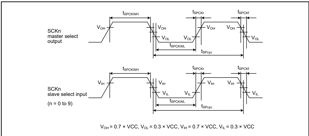
Figure 2.42 SCKn simple SPI mode clock timing
