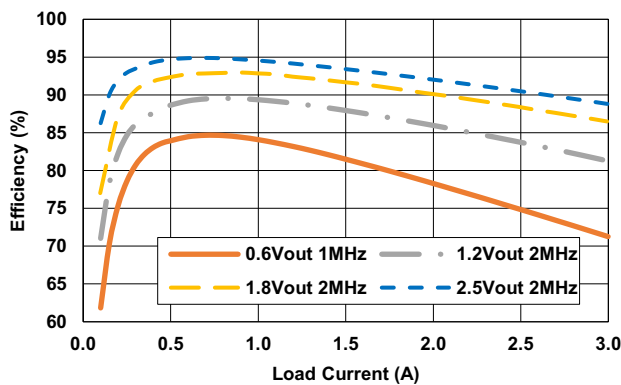
Figure 5. V IN = 3.3V, FPWM
