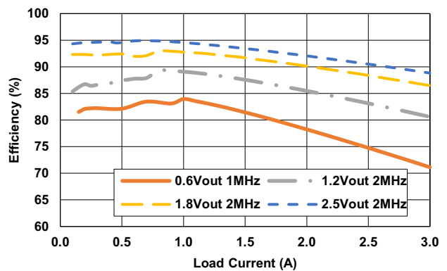
Figure 6. V IN = 3.3V, PFM
