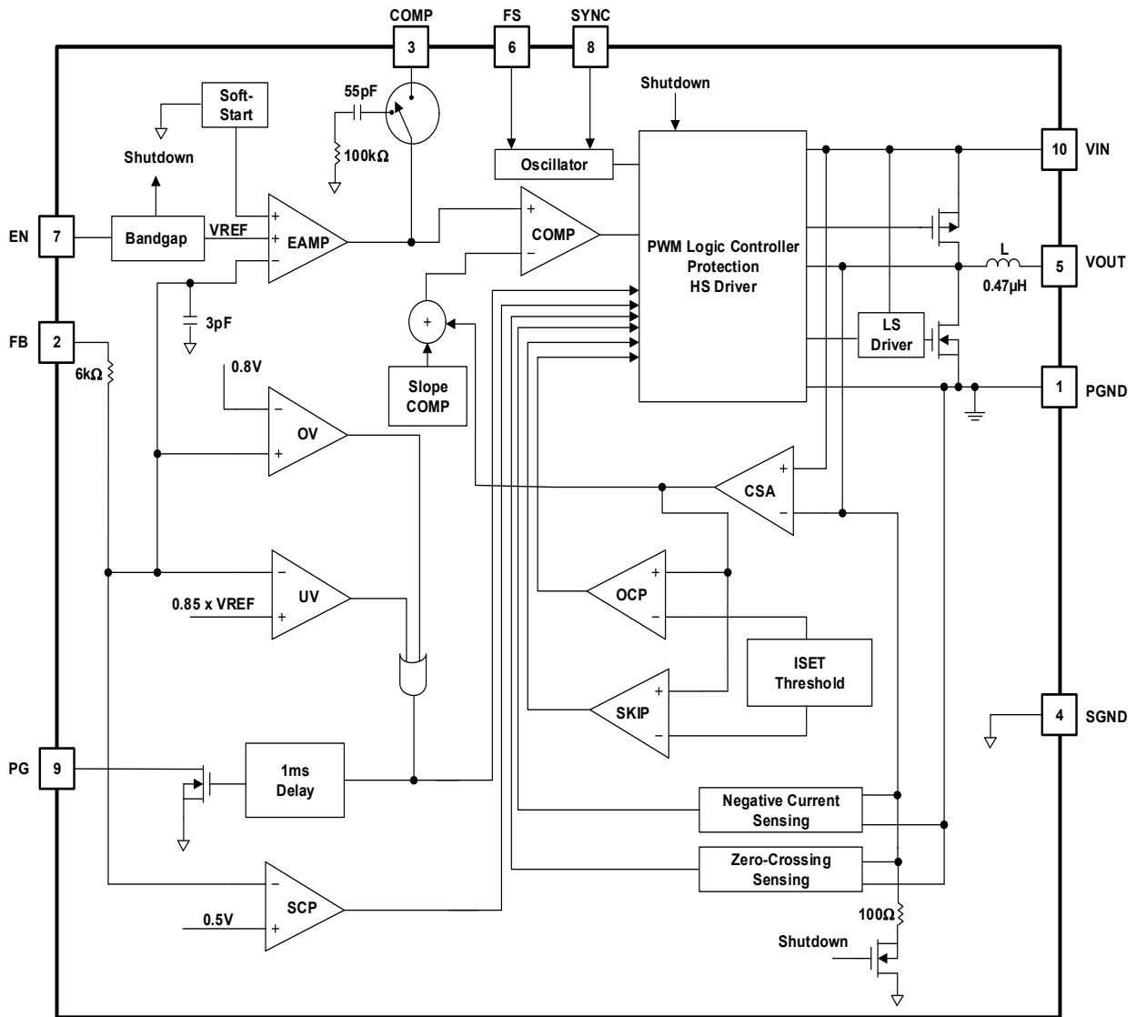
Figure 4. Block Diagram
