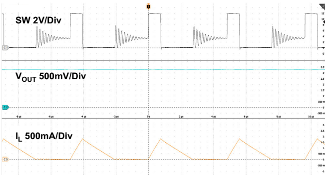
Figure 12. Steady-State Operation, I_{OUT} = 1\text{A} ( V_{OUT} = 3.3\text{V} )
