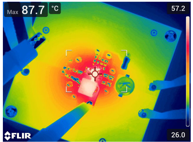
Figure 41. 12\text{V}_{IN} , 5\text{V}_{OUT} , 3A load, IC Temperature = 87.7^\circ\text{C} , Max Ambient Temperature = 60.3^\circ\text{C}
