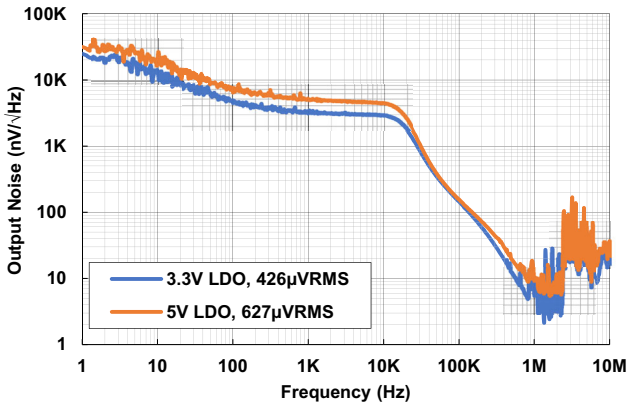
Figure 29. Output Noise vs Frequency V OUT = V INLDO = 6V, C OUT = 4.7μF,0.1μF
