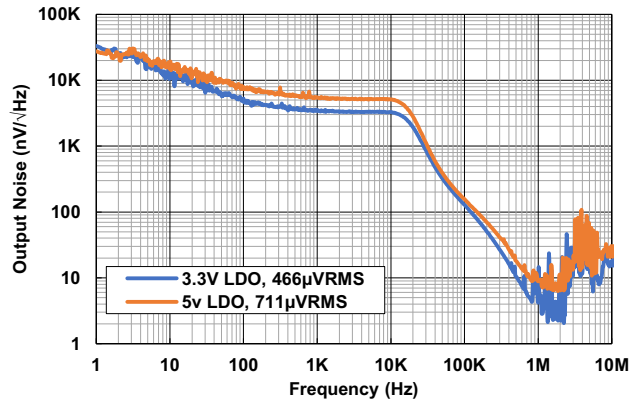
Figure 30. Output Noise vs Frequency V OUT = V INLDO = 12V, C OUT = 4.7μF,0.1μF
