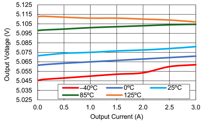
Figure 30. Load Regulation vs Output Current ( V_{OUT} = 5.1\text{V} )
