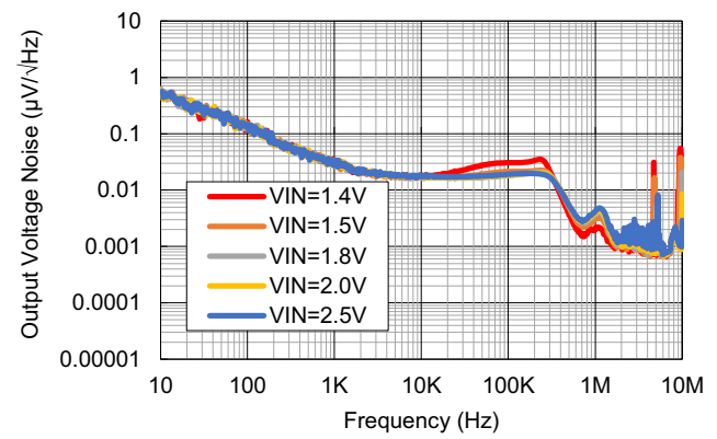
Figure 13. Output Voltage Noise for Various V_{IN} ( V_{OUT} = 0.5\text{V} , I_{OUT} = 3\text{A} )
