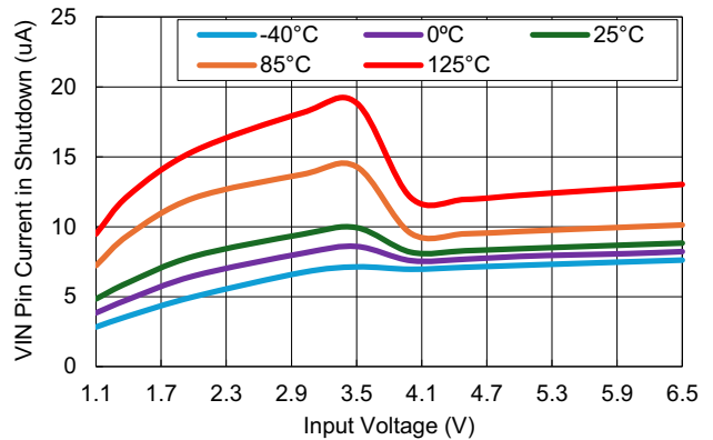
Figure 40. Shutdown Current vs Input Voltage for Various Temperatures
