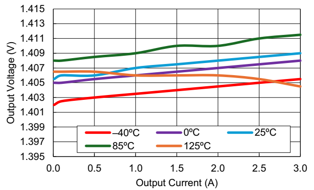
Figure 28. Load Regulation vs Output Current ( V_{OUT} = 1.4\text{V} )
