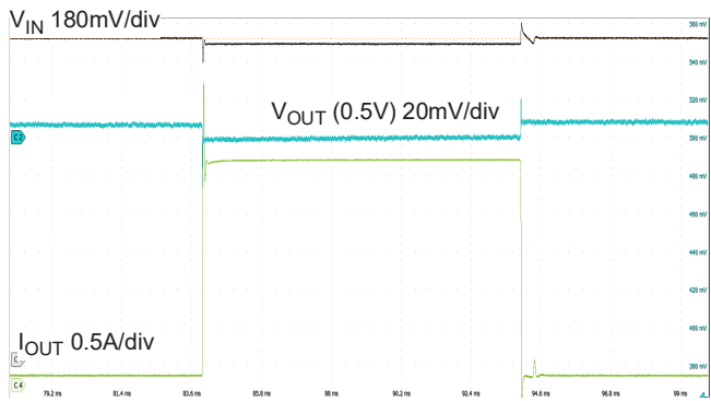
Figure 21. Load Transient Response for ( V_{IN} = 1.4\text{V} , V_{OUT} = 0.5\text{V} , \Delta I_{OUT} = 0.1\text{mA} to 3\text{A} at 1\text{A}/\mu\text{s} )
