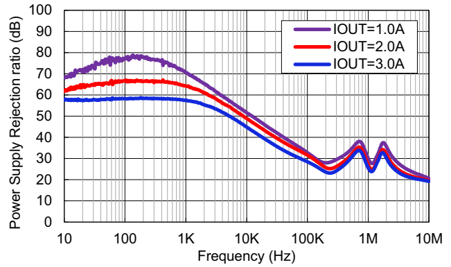
Figure 5. PSRR vs Frequency for Various I_{OUT} ( V_{IN} = 1.1\text{V} , V_{OUT} = 0.8\text{V} , V_{BIAS} = 5\text{V} , C_{NR/SS} = 0.1\mu\text{F} )
