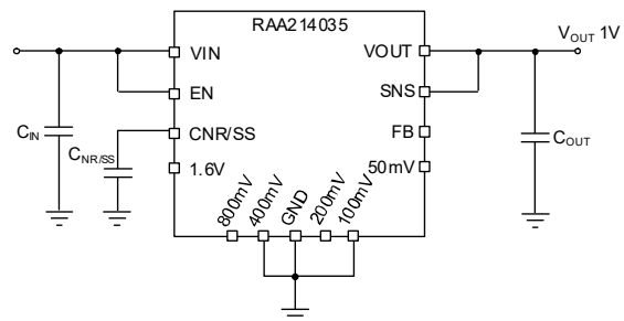
Figure 45. Internal FB Resistor Configuration for 1V ( V_{OUT} = 0.5V_{REF} + 400mV + 100mV )
