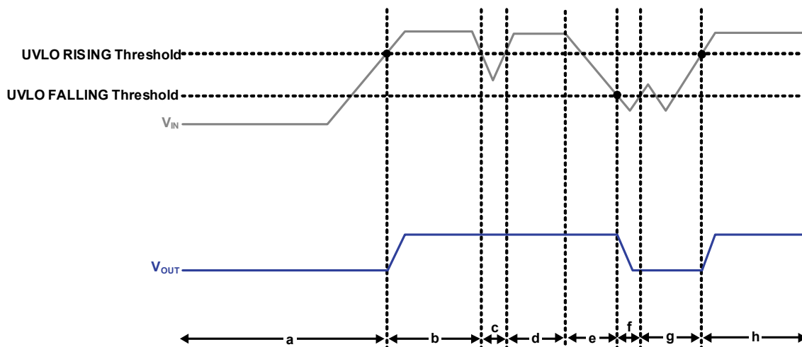
Figure 43. UVLO Operation
