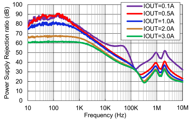
Figure 7. PSRR vs Frequency for Various I_{OUT} ( V_{IN} = 3.7\text{V} , V_{OUT} = 3.3\text{V} )
