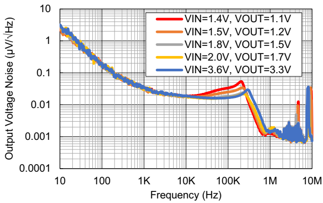
Figure 8. Output Voltage Noise for Various V_{OUT} ( V_{IN} = V_{OUT} + 0.3\text{V} , I_{OUT} = 3\text{A} , C_{NR/SS} = 0.1\mu\text{F} )
