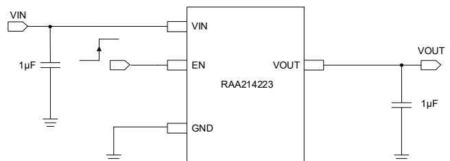
Figure 2. RAA214223 Typical Application (2)
