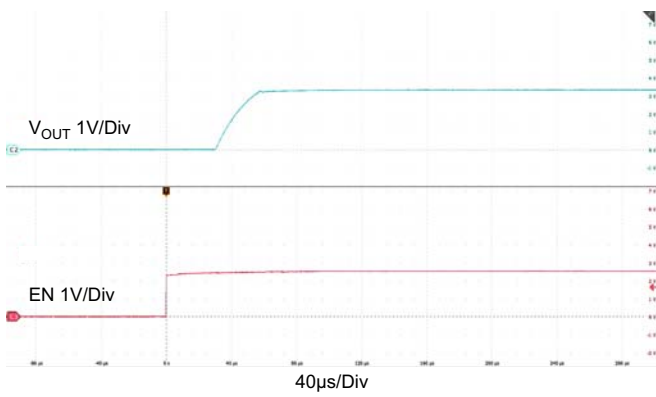
Figure 12. Startup with EN ( I_{OUT} = 150mA )
