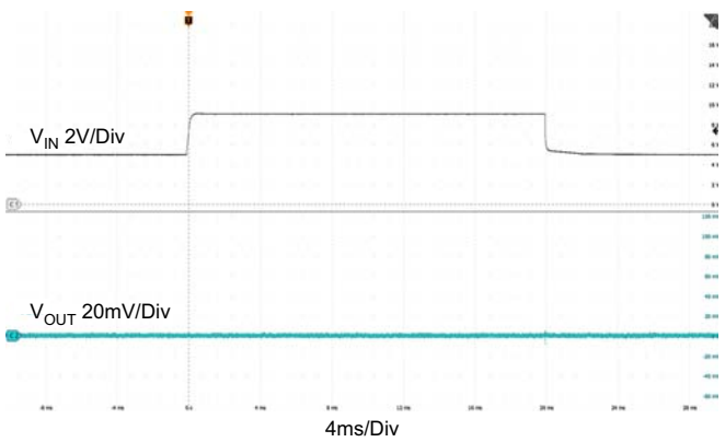
Figure 17. Line Transient (5V to 12V, C_{OUT} = 1\mu F , I_{OUT} = 10mA )
