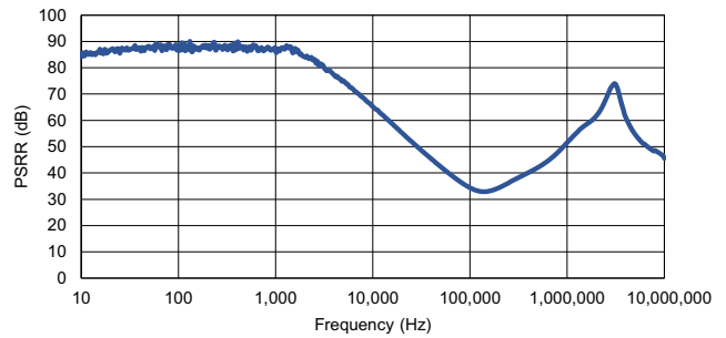
Figure 15. PSRR ( V_{IN} = 5V , I_{OUT} = 10mA )
