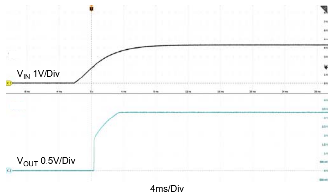
Figure 13. Startup with VIN ( I_{OUT} = 150mA )
