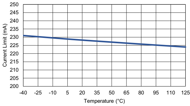
Figure 10. Current Limit vs Temperature
