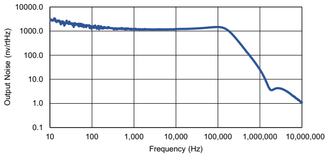
Figure 14. Output Noise Spectral Density ( V_{IN} = 5V , I_{OUT} = 10mA )
