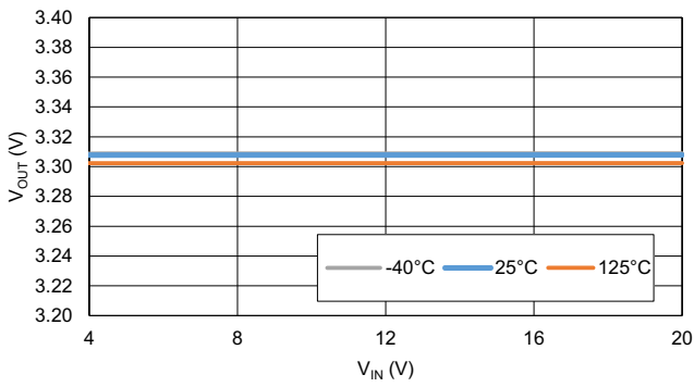
Figure 8. Output Voltage vs Input Voltage ( I_{OUT} = 1mA )
