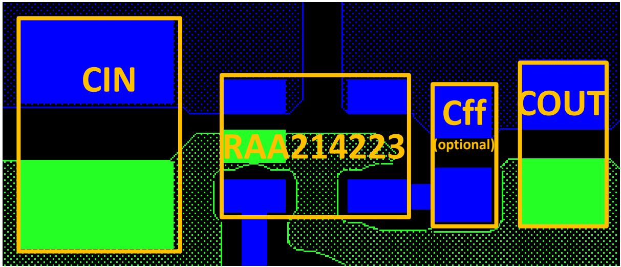
Figure 18. Recommended Component Placement
