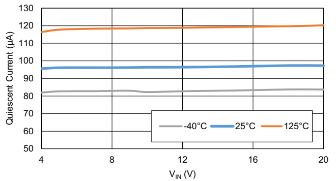
Figure 5. Quiescent Current (No Load) vs Input Voltage
