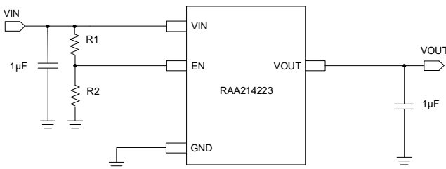
Figure 1. RAA214223 Typical Application (1)
