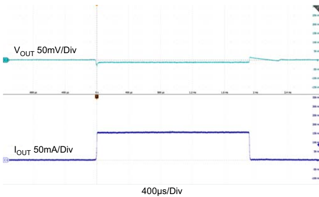
Figure 16. Load Transient (0 to 150mA, C_{OUT} = 1\mu F )
