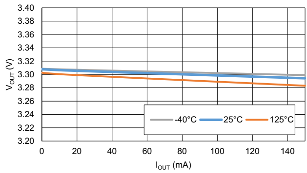
Figure 9. Output Voltage vs Load
