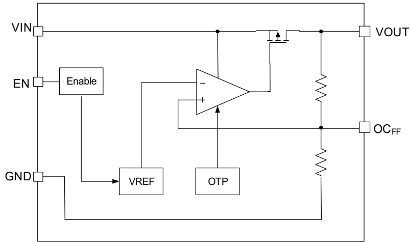
Figure 3. Block Diagram
