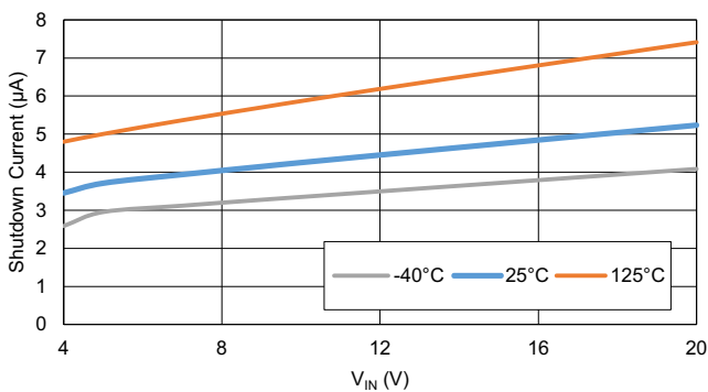
Figure 6. Shutdown Current (EN = 0) vs Input Voltage
