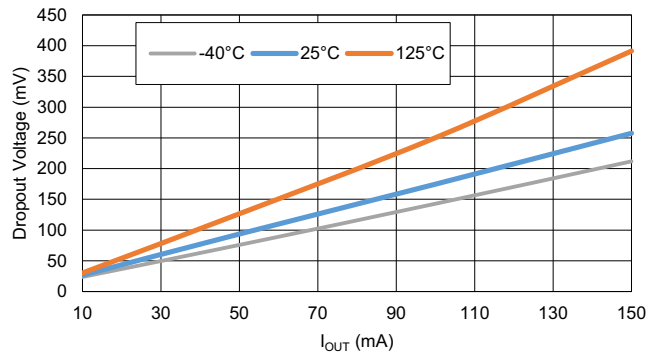
Figure 11. Dropout Voltage vs Load
