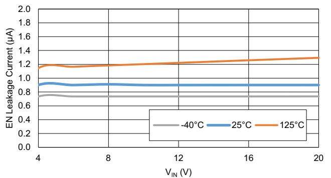
Figure 7. EN Leakage Current vs Temperature
