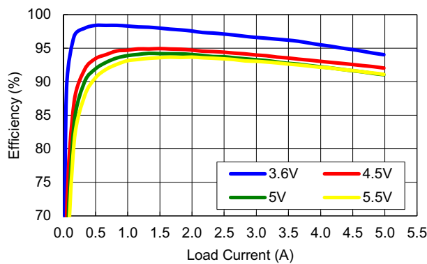
Figure 14. Efficiency vs Load, V OUT = 3.3V, L = 0.47µH
