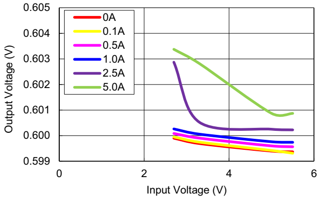
Figure 20. Line Regulation, V_{OUT} = 0.6V
