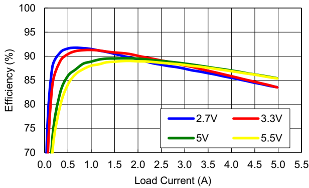
Figure 12. Efficiency vs Load, V OUT = 1.8V, L = 0.47µH
