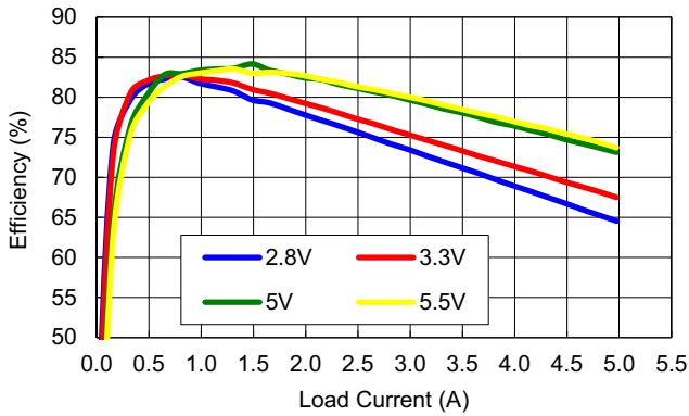
Figure 10. Efficiency vs Load, V OUT = 0.6V, L = 0.47µH
