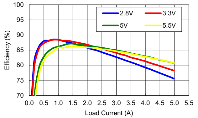
Figure 11. Efficiency vs Load, V OUT = 1.2V, L = 0.47µH
