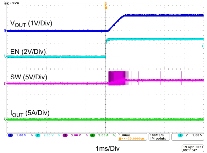
Figure 34. EN On at No Load
