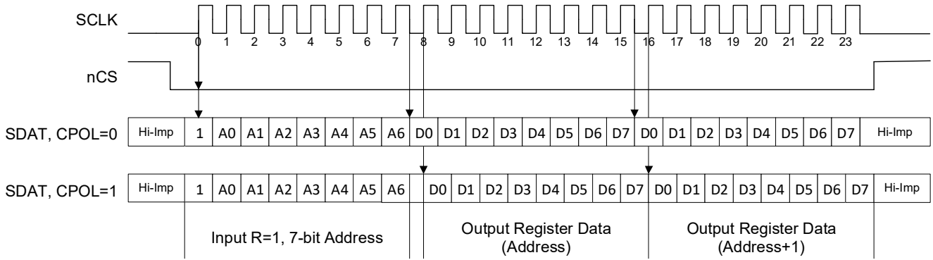
Figure 9. Logic Diagram: READ Data from RC18008 Registers for CPOL = 0 and CPOL = 1
