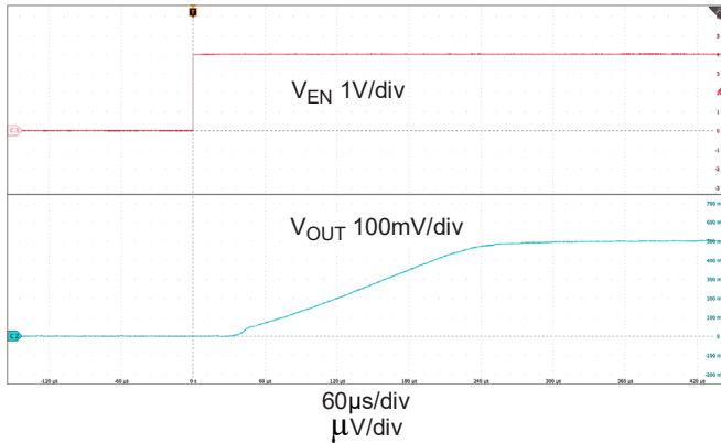
Figure 14. Start-Up ( V_{IN} = 1.1\text{V} , V_{OUT} = 0.5\text{V} , V_{BIAS} = 5\text{V} , I_{OUT} = 4\text{A} , C_{NR/SS} = 1\mu\text{F} )
