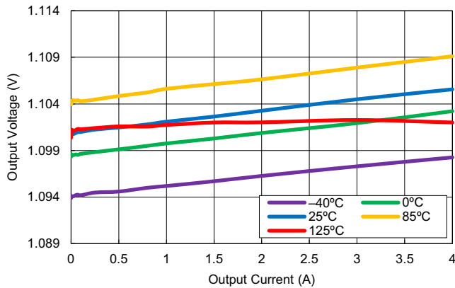
Figure 32. Load Regulation vs Output Current ( V_{IN} = 1.5\text{V} , V_{OUT} = 1.1\text{V} )
