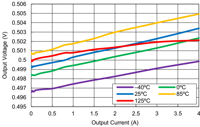
Figure 30. Load Regulation vs Output Current ( V_{IN} = 1.1\text{V} , V_{BIAS} = 5\text{V} , V_{OUT} = 0.5\text{V} )
