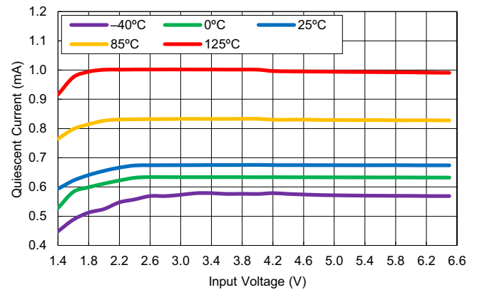
Figure 39. Quiescent Current vs Input Voltage for Various Temperatures
