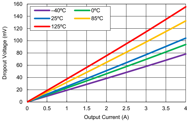
Figure 24. Dropout Voltage vs Output Current ( V_{OUT} = 1.1\text{V} , V_{BIAS} = 5\text{V} )
