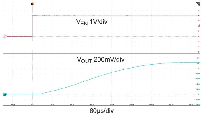
Figure 17. Start-Up ( V_{IN} = 1.5\text{V} , V_{OUT} = 1.2\text{V} , I_{OUT} = 4\text{A} , C_{NR/SS} = 1\mu\text{F} )
