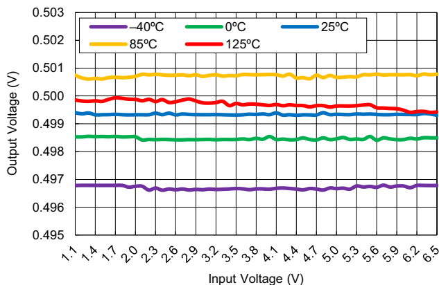
Figure 34. Line Regulation vs Input Voltage ( V_{BIAS} = 5\text{V} , V_{OUT} = 0.5\text{V} , I_{OUT} = 5\text{mA} )
