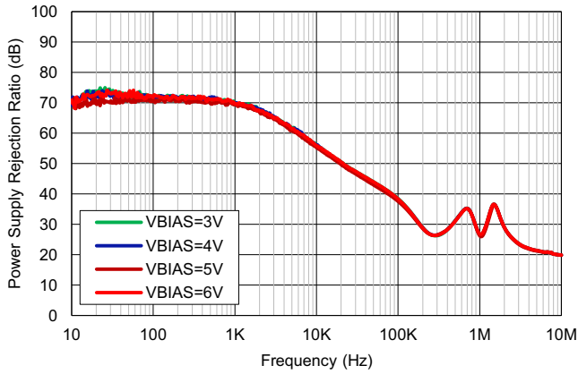
Figure 4. PSRR vs Frequency for Various BIAS ( V_{IN} = 1.1\text{V} , V_{OUT} = 0.5\text{V} , I_{OUT} = 4\text{A} , C_{NR/SS} = 1\mu\text{F} )
