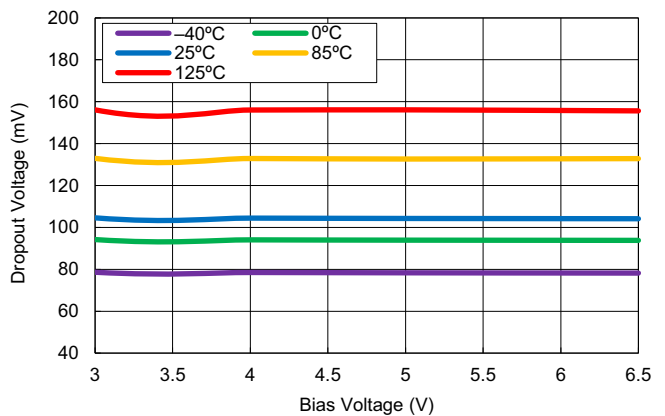
Figure 29. Dropout Voltage vs BIAS Voltage ( V_{IN} = 1.4\text{V} , I_{OUT} = 4\text{A} )
