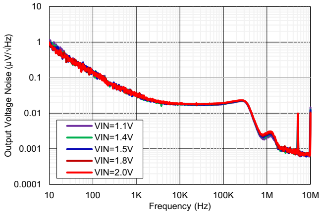
Figure 9. Output Voltage Noise for Various V_{IN} ( V_{OUT} = 0.5\text{V} , V_{BIAS} = 5\text{V} , I_{OUT} = 4\text{A} , C_{NR/SS} = 1\mu\text{F} )
