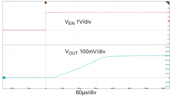
Figure 15. Start-Up ( V_{IN} = 1.4\text{V} , V_{OUT} = 0.5\text{V} , I_{OUT} = 4\text{A} , C_{NR/SS} = 1\mu\text{F} )
