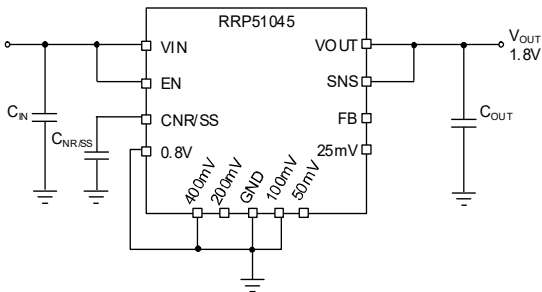
Figure 52. Internal FB Resistor Configuration for 1.8V (V_{OUT} = 0.5V_{REF} + 800mV + 400mV + 100mV)
