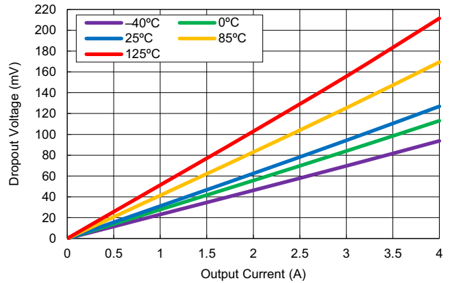
Figure 25. Dropout Voltage vs Output Current ( V_{OUT} = 1.4\text{V} without BIAS)
