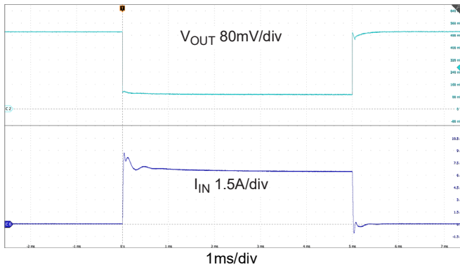
Figure 22. Short Circuit after Start-Up ( V_{IN} = 1.4\text{V} , V_{OUT} = 0.5\text{V} , C_{NR/SS} = 1\mu\text{F} )
