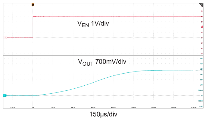
Figure 19. Start-Up ( V_{IN} = 3.6\text{V} , V_{OUT} = 3.3\text{V} , I_{OUT} = 4\text{A} , C_{NR/SS} = 1\mu\text{F} )
