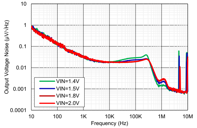
Figure 10. Output Voltage Noise for Various V_{IN} ( V_{OUT} = 0.5\text{V} , I_{OUT} = 4\text{A} , C_{NR/SS} = 1\mu\text{F} )
