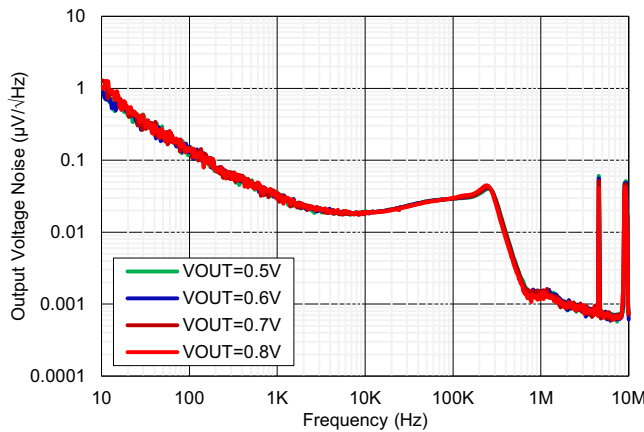
Figure 11. Output Voltage Noise for Various V_{OUT} ( V_{IN} = 1.4\text{V} , I_{OUT} = 4\text{A} , C_{NR/SS} = 1\mu\text{F} )
