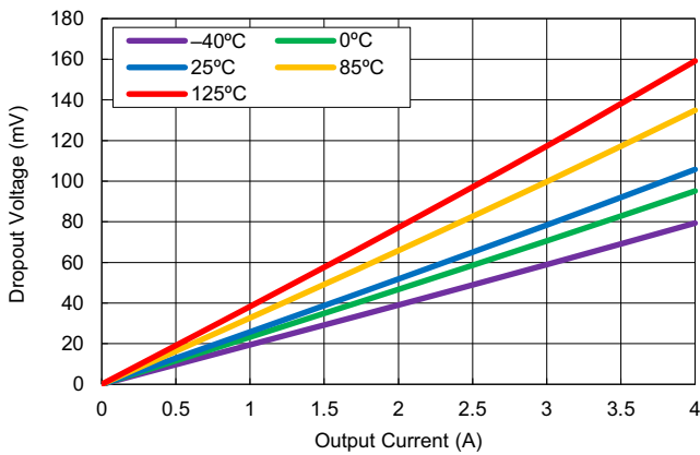
Figure 26. Dropout Voltage vs Output Current ( V_{IN} = 3.5\text{V} without BIAS)
