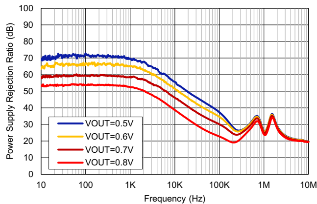
Figure 8. PSRR vs Frequency for Various V_{OUT} ( V_{IN} = 1.1\text{V} , V_{BIAS} = 5\text{V} , I_{OUT} = 4\text{A} , C_{NR/SS} = 1\mu\text{F} )
