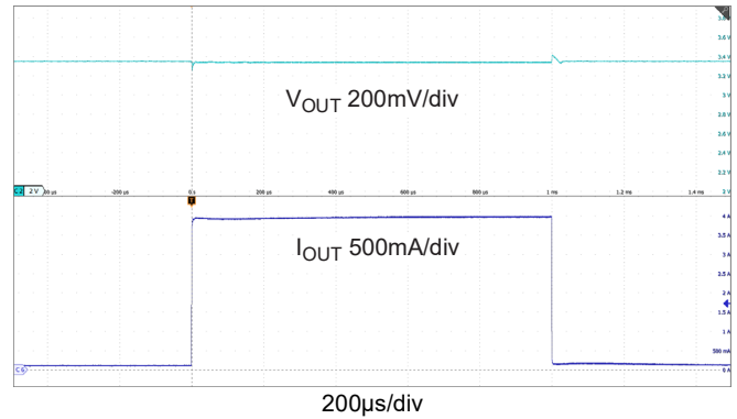
Figure 21. Load Transient Response ( V_{IN} = 3.7\text{V} , V_{OUT} = 3.3\text{V} , \Delta I_{OUT} = 0.1\text{A} to 4\text{A} at 1\text{A}/\mu\text{s} , C_{NR/SS} = 1\mu\text{F} )
