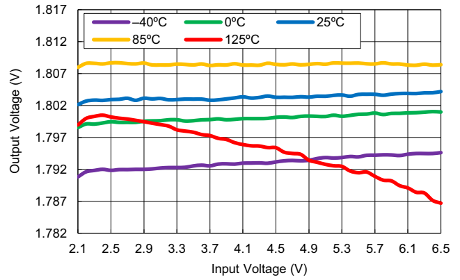
Figure 37. Line Regulation vs Input Voltage ( V_{OUT} = 1.8\text{V} , I_{OUT} = 5\text{mA} )
