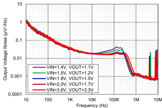
Figure 13. Output Voltage Noise for Various V_{OUT} ( V_{IN} = V_{OUT} + 0.3\text{V} , I_{OUT} = 4\text{A} , C_{NR/SS} = 1\mu\text{F} )
