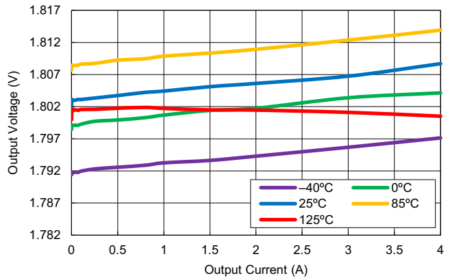
Figure 33. Load Regulation vs Output Current ( V_{OUT} = 2.2\text{V} , V_{OUT} = 1.8\text{V} )
