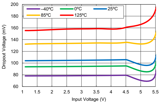
Figure 28. Dropout Voltage vs Input Voltage ( V_{BIAS} = 6.5\text{V} , I_{OUT} = 4\text{A} )
