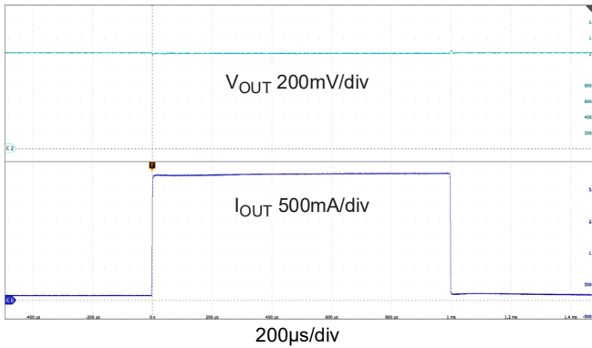
Figure 20. Load Transient Response ( V_{IN} = 1.6\text{V} , V_{OUT} = 1.2\text{V} , \Delta I_{OUT} = 0.1\text{A} to 4\text{A} at 1\text{A}/\mu\text{s} , C_{NR/SS} = 1\mu\text{F} )
