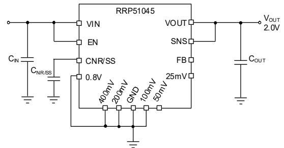
Figure 53. Internal FB Resistor Configuration for 2.0V (V_{OUT} = 0.5V_{REF} + 800mV + 400mV + 200mV + 100mV)
