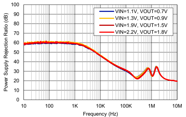
Figure 7. PSRR vs Frequency for Various V_{OUT} ( V_{IN} = V_{OUT} + 0.4\text{V} , V_{BIAS} = 5\text{V} , I_{OUT} = 4\text{A} , C_{NR/SS} = 1\mu\text{F} )
