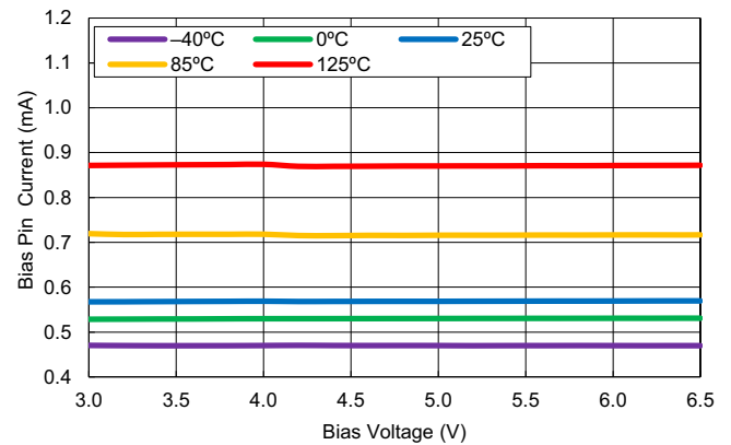
Figure 41. Bias Pin Quiescent Current vs Bias Voltage for Various Temperatures ( V_{IN} = 1.1\text{V} )
