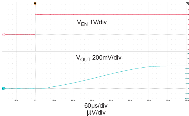
Figure 16. Start-Up ( V_{IN} = 1.4\text{V} , V_{OUT} = 0.9\text{V} , I_{OUT} = 4\text{A} , C_{NR/SS} = 1\mu\text{F} )
