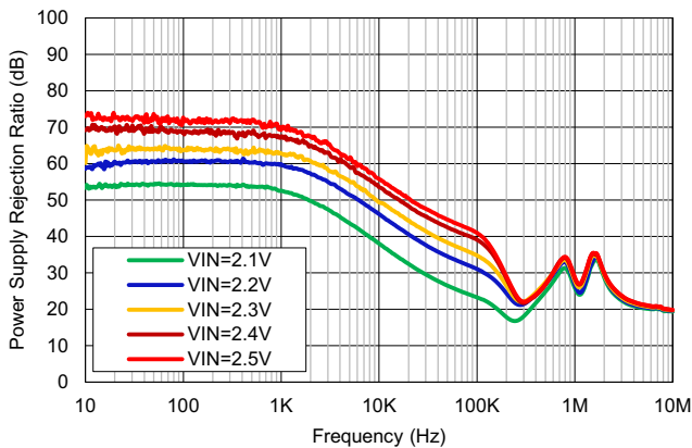
Figure 6. PSRR vs Frequency for Various V_{IN} ( V_{OUT} = 1.8\text{V} , I_{OUT} = 4\text{A} , C_{NR/SS} = 1\mu\text{F} )
