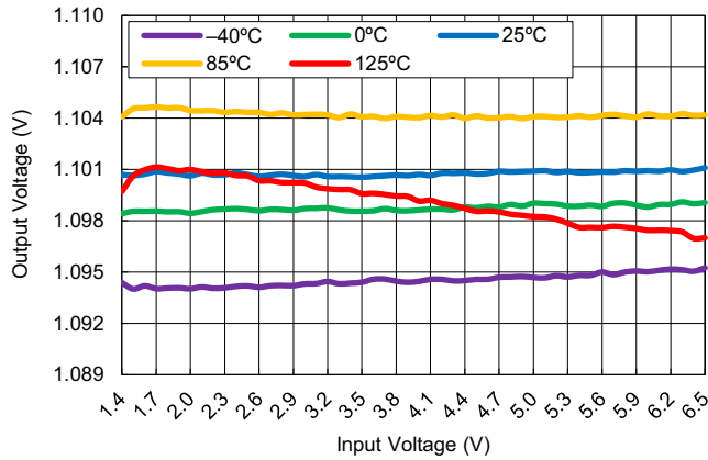
Figure 36. Line Regulation vs Input Voltage ( V_{OUT} = 1.1\text{V} , I_{OUT} = 5\text{mA} )
