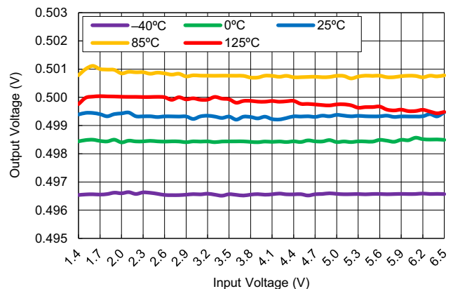
Figure 35. Line Regulation vs Input Voltage ( V_{OUT} = 0.5\text{V} , I_{OUT} = 5\text{mA} )
