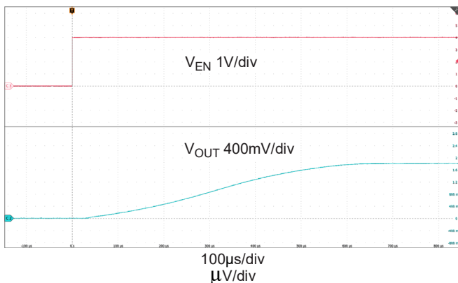
Figure 18. Start-Up ( V_{IN} = 2.1\text{V} , V_{OUT} = 1.8\text{V} , I_{OUT} = 4\text{A} , C_{NR/SS} = 1\mu\text{F} )
