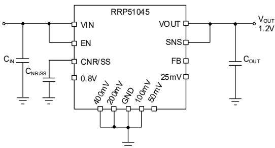
Figure 50. Internal FB Resistor Configuration for 1.2V (V_{OUT} = 0.5V_{REF} + 400mV + 200mV + 100mV)
