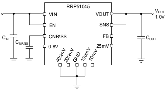
Figure 48. Internal FB Resistor Configuration for 1.0V (V_{OUT} = 0.5V_{REF} + 400mV + 100mV)
