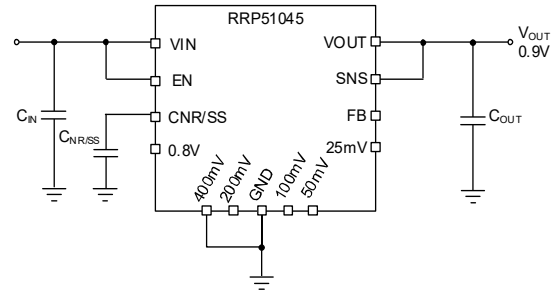
Figure 47. Internal FB Resistor Configuration for 0.9V (V_{OUT} = 0.5V_{REF} + 400mV)
