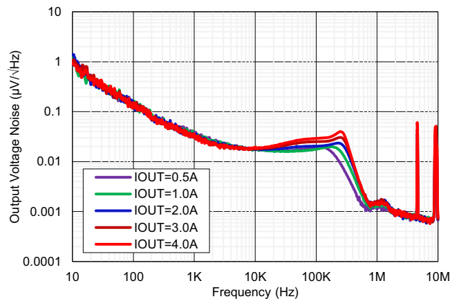
Figure 12. Output Voltage Noise for Various I_{OUT} ( V_{IN} = 1.4\text{V} , V_{OUT} = 0.5\text{V} , C_{NR/SS} = 1\mu\text{F} )
