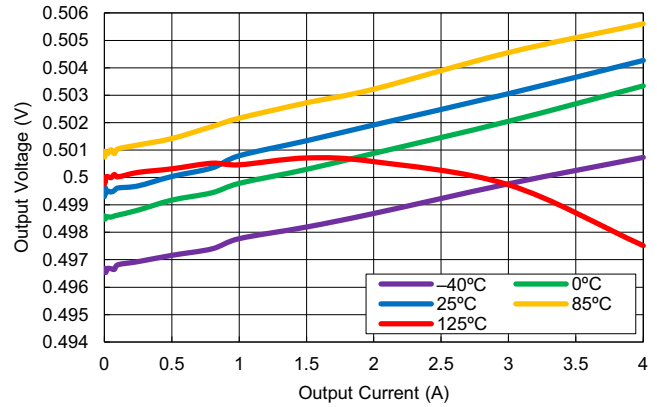
Figure 31. Load Regulation vs Output Current ( V_{IN} = 1.4\text{V} , V_{OUT} = 0.5\text{V} )
