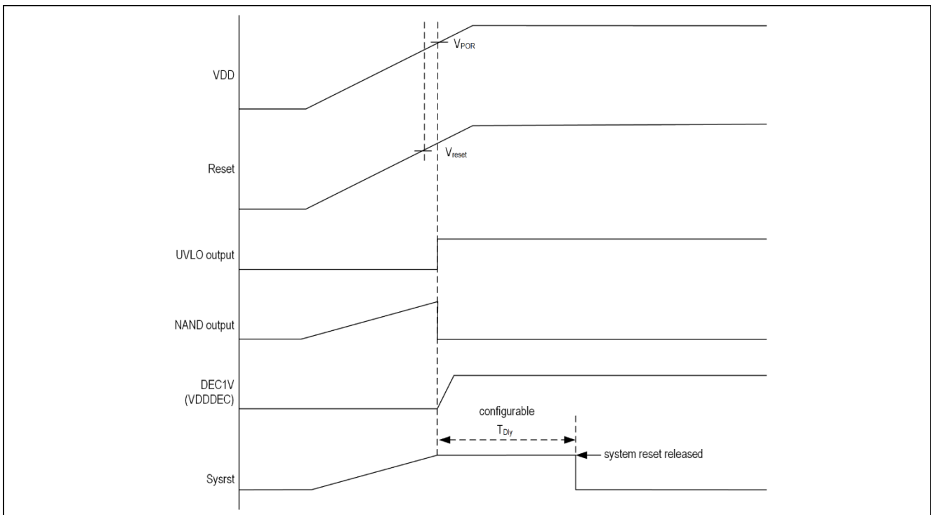
Figure 2. Power-up sequence
