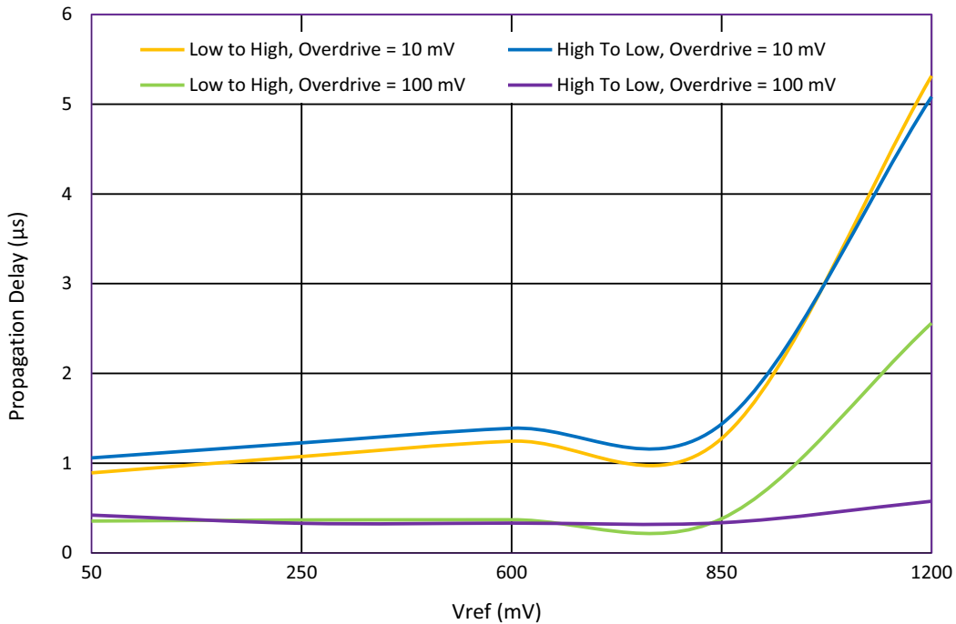
Figure 61. ACMPx Typical Propagation Delay at T_A = +25^\circ\text{C} , Gain = 1, Hysteresis = 0, V_{DD} = 1.71\text{ V to }5.5\text{ V} , LPF-Disable
