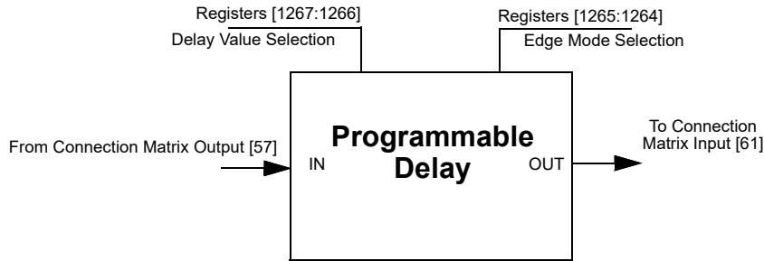
Figure 64. Programmable Delay
