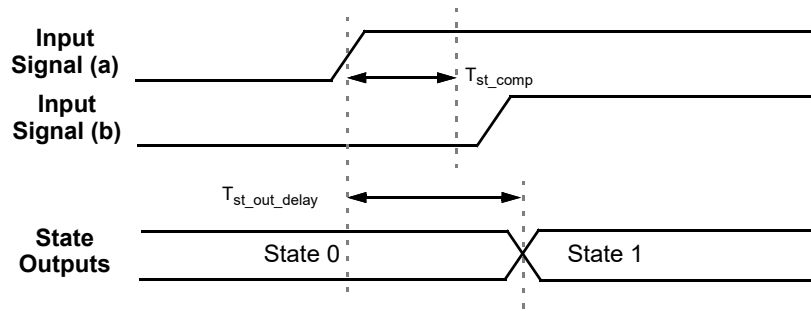
Figure 111. State Transition Timing - Competing Inputs Determinable
