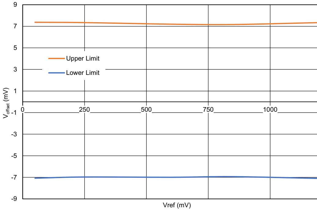
Figure 58. ACMPx Input Offset Voltage vs. V REF at V DD = 1.71 V to 5.5 V, T A = -40 °C to +105 °C
