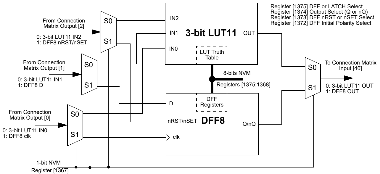
Figure 23. 3-bit LUT11 or DFF8 with RST/SET
