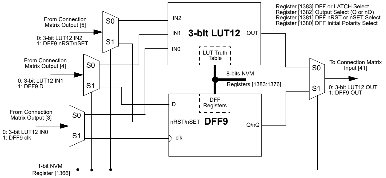
Figure 24. 3-bit LUT12 or DFF9 with RST/SET
