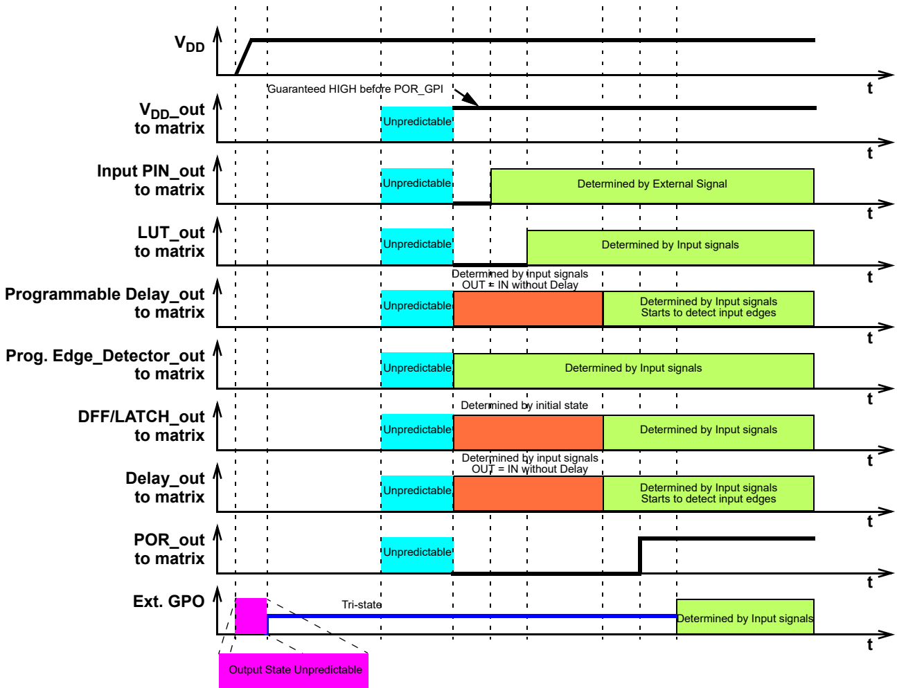
Figure 95. Internal Macrocell States during POR Sequence
