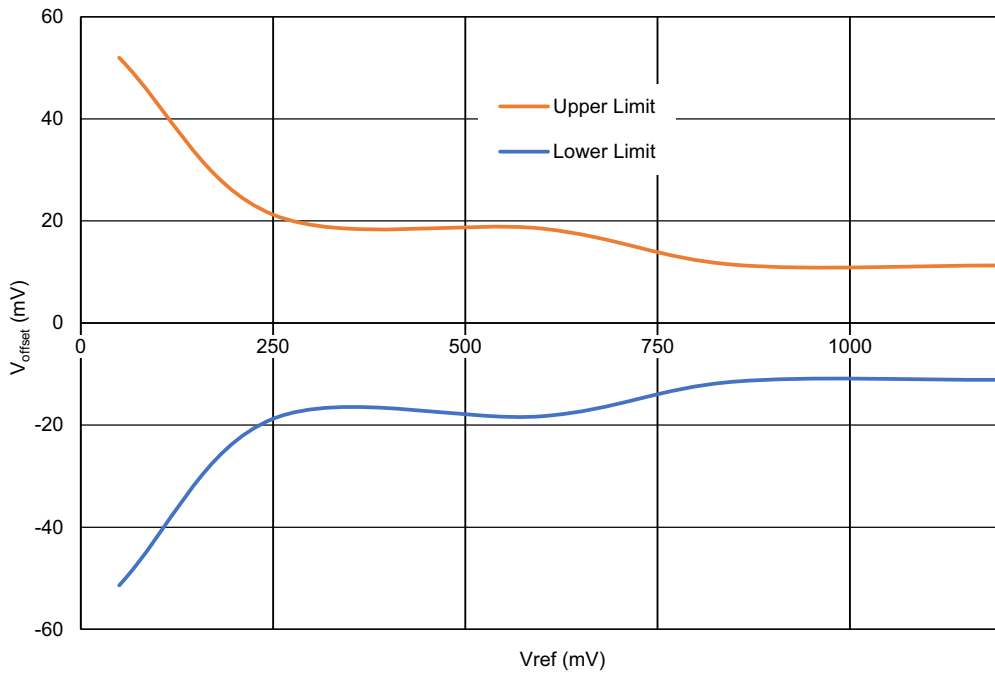
Figure 59. ACMPx Buffer Input Offset Voltage vs. V REF at V DD = 1.71 V to 5.5 V, T A = -40 °C to +105 °C
