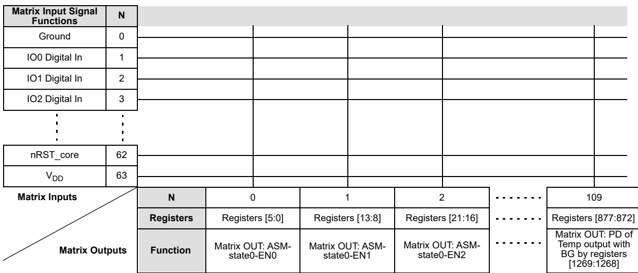
Figure 12. Connection Matrix
