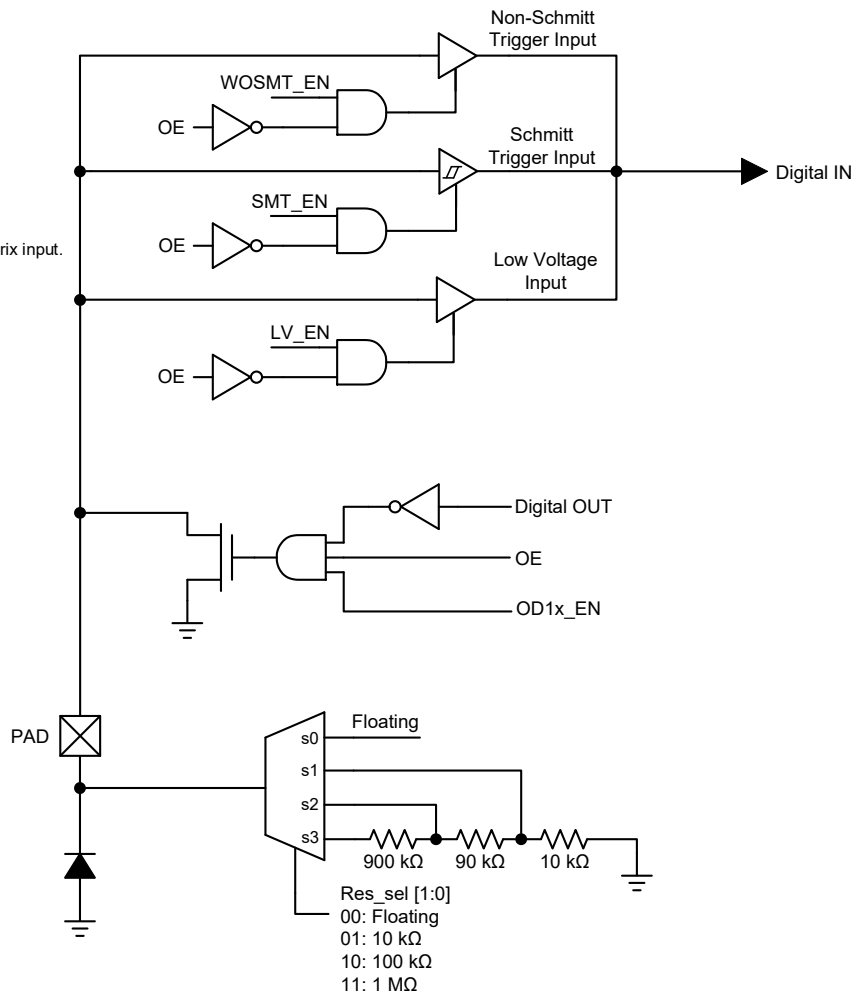
Figure 7. Matrix OE IO Structure Diagram
