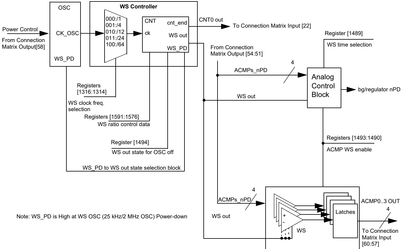
Figure 52. Wake/Sleep Controller
