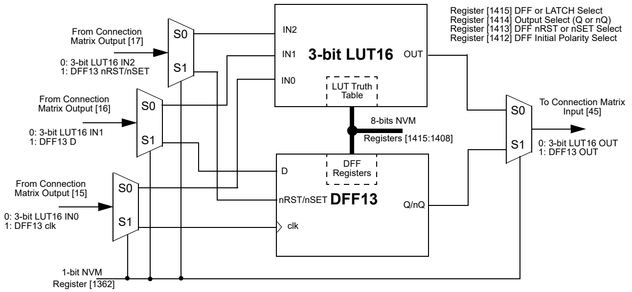
Figure 28. 3-bit LUT16 or DFF13 with RST/SET
