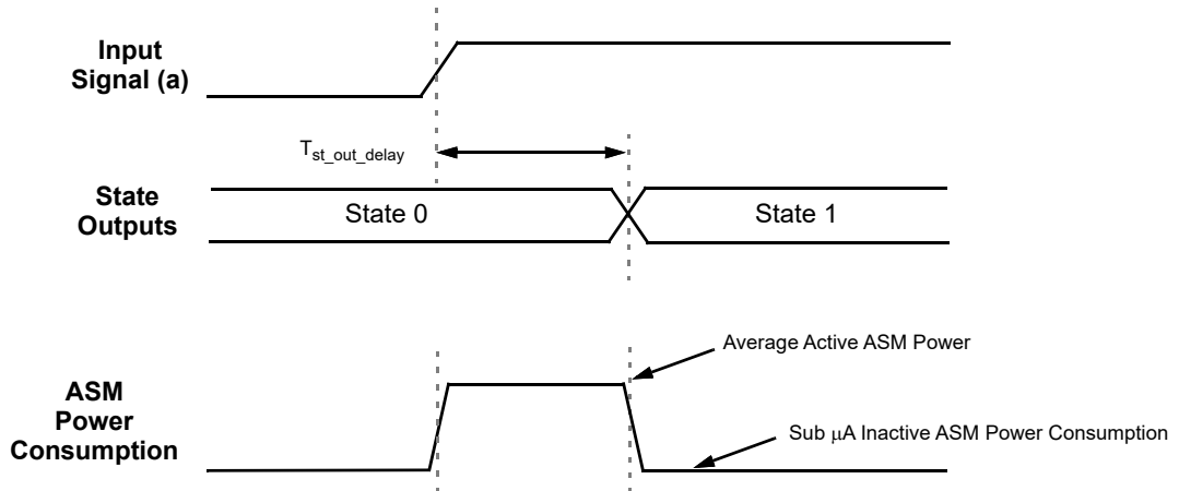
Figure 106. State Transition Timing and Power Consumption
