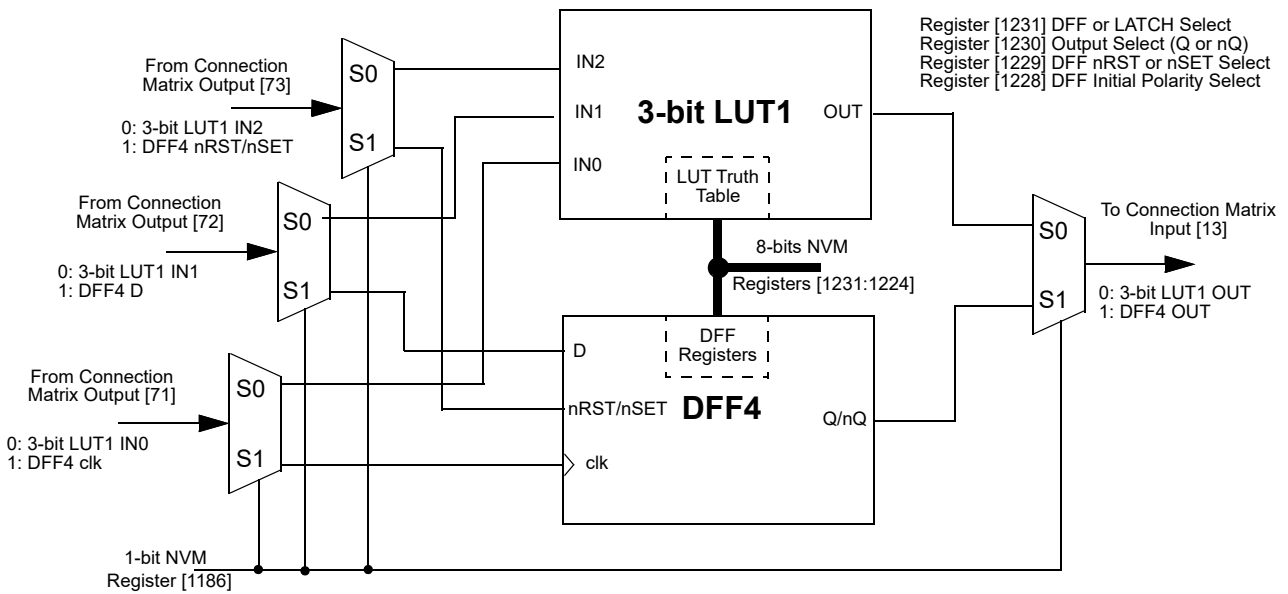
Figure 19. 3-bit LUT1 or DFF4 with RST/SET
