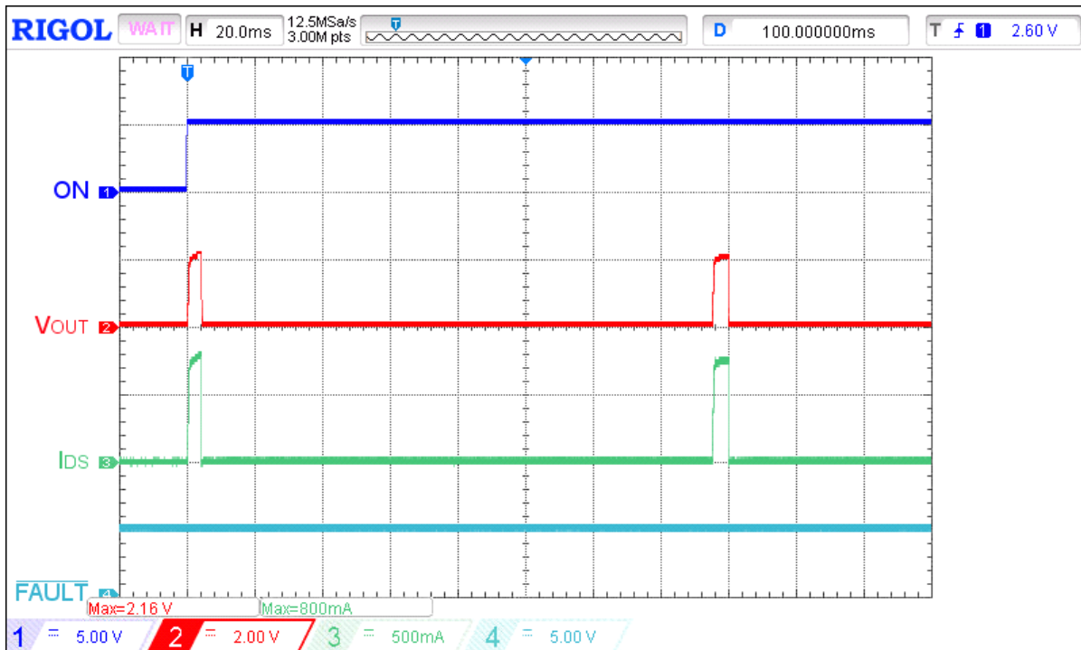
Figure 23. Extended typical SOA waveform during powerup on heavy load for V_{IN} = 9\text{ V} , C_{LOAD} = 10\ \mu\text{F} , R_{SET} = 30.1\ \text{k}\Omega , R_{LOAD} = 3.8\ \Omega
