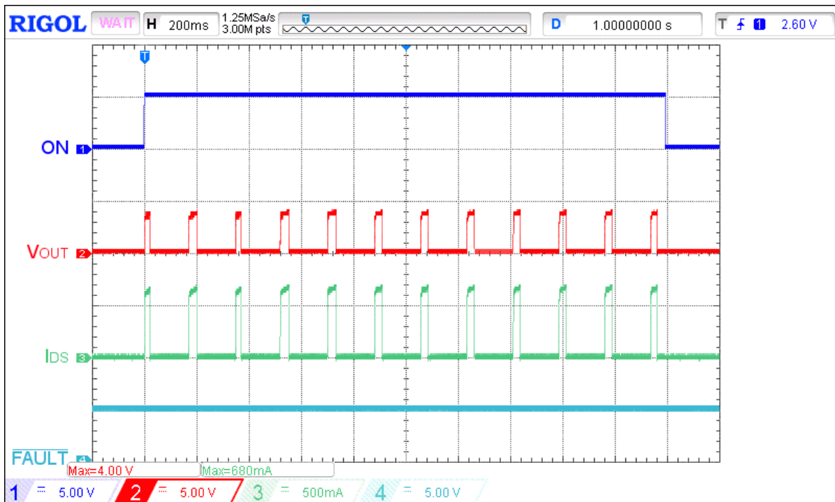
Figure 24. Typical SOA waveform during powerup on heavy load for V_{IN} = 12\text{ V} , C_{LOAD} = 10\ \mu\text{F} , R_{SET} = 30.1\ \text{k}\Omega , R_{LOAD} = 3.8\ \Omega
