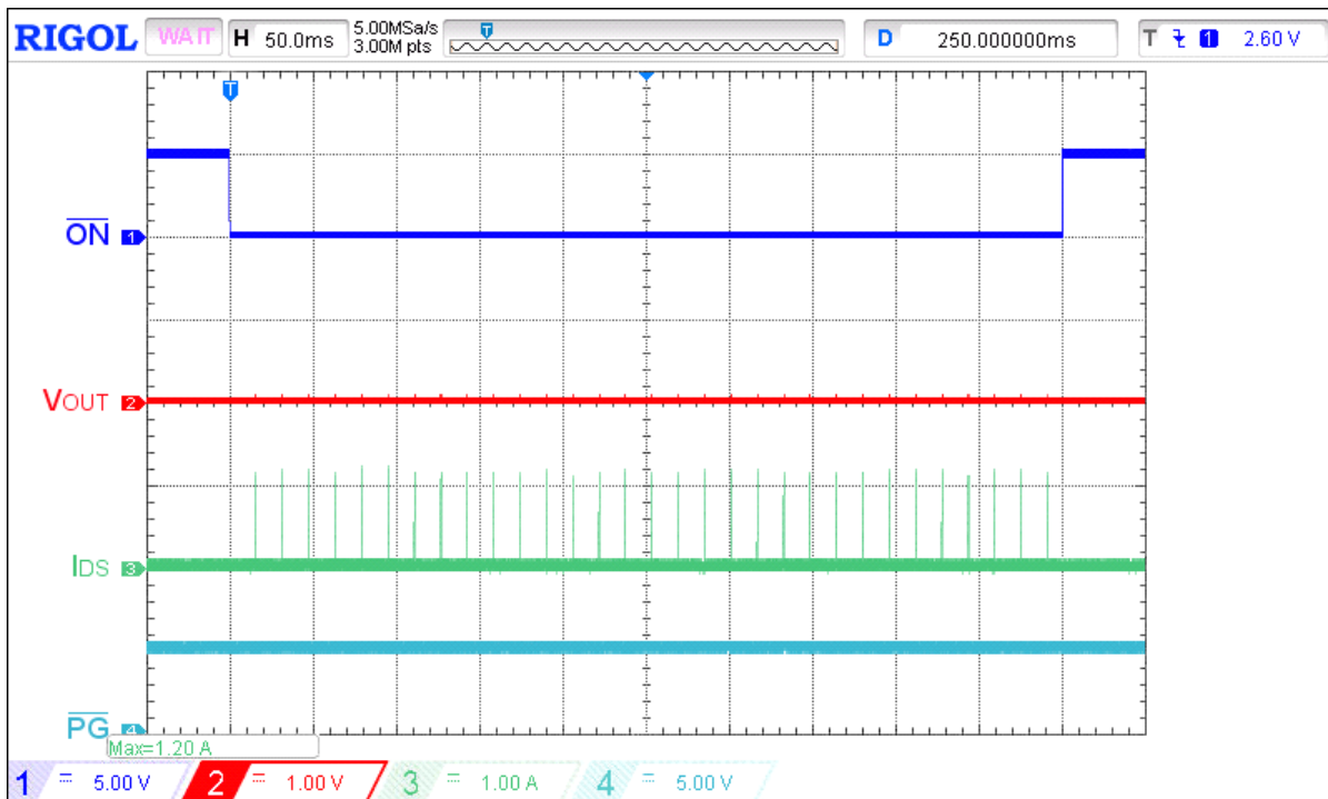
Figure 24. Startup Current Protection operation waveform for V_{\text{IN}} = 12 \text{ V}
