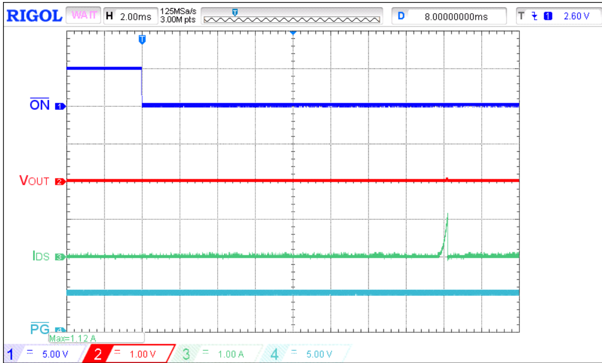
Figure 23. Startup Current Protection operation waveform for V_{\text{IN}} = 9 \text{ V} (extended view)
