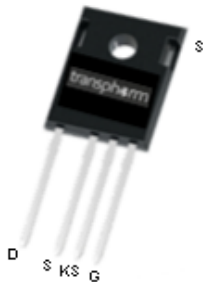
TP65H050G4YS TO-247 (top view)
