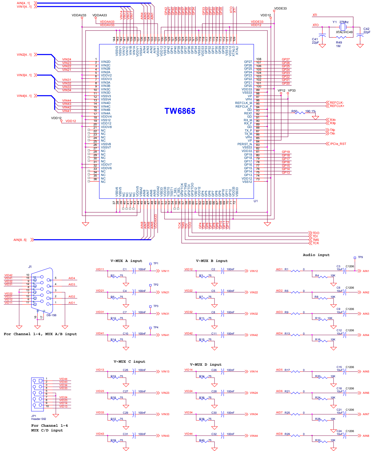
FIGURE 11. TW6865 APPLICATION SCHEMATIC
